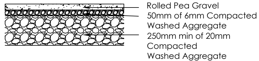
Section 1:20
