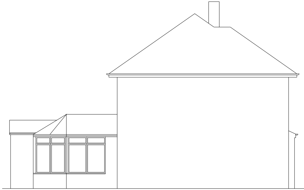
EXISTING ANOTHER SIDE ELEVATION
