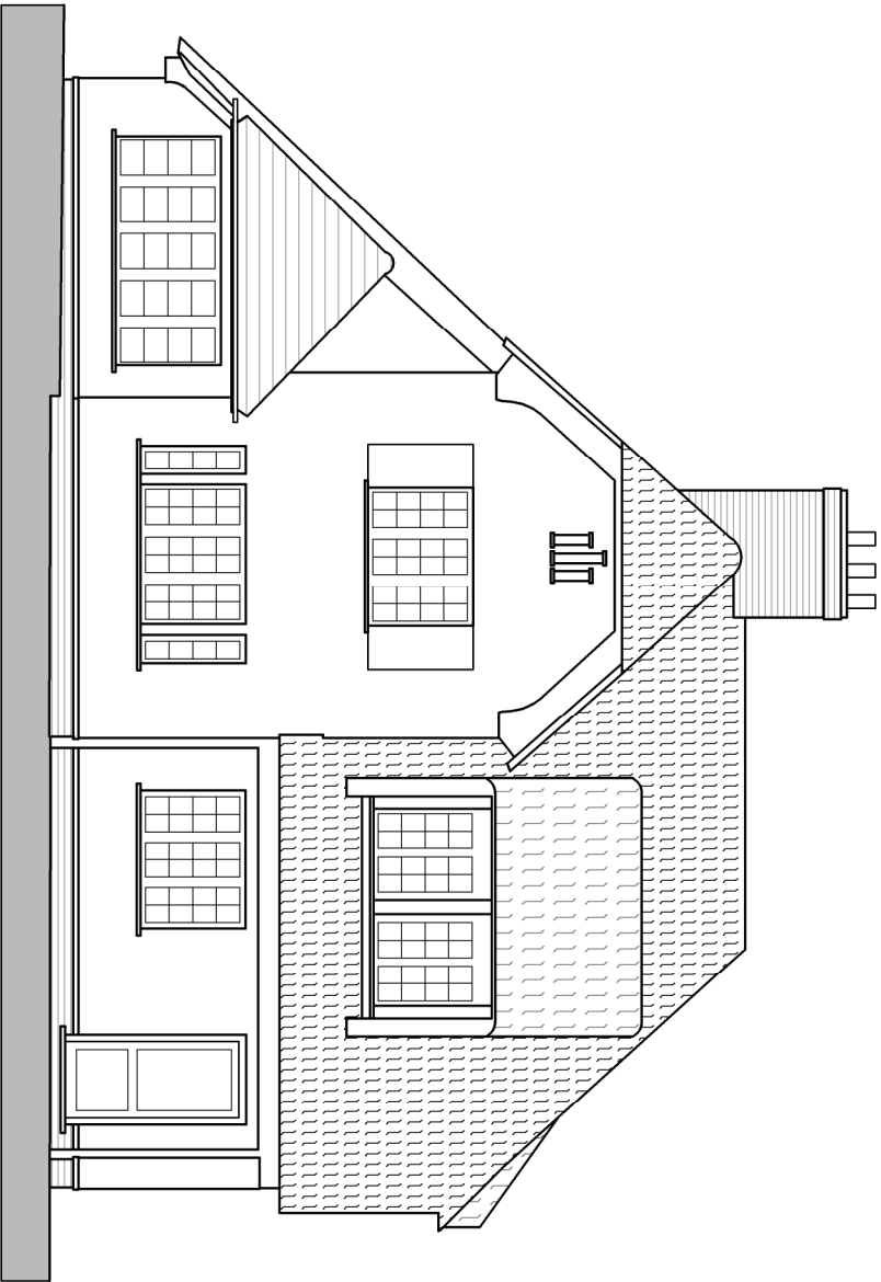
West (Rear) Elevation
