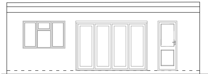
PROPOSED WEST ELEVATION Scale 1:100
