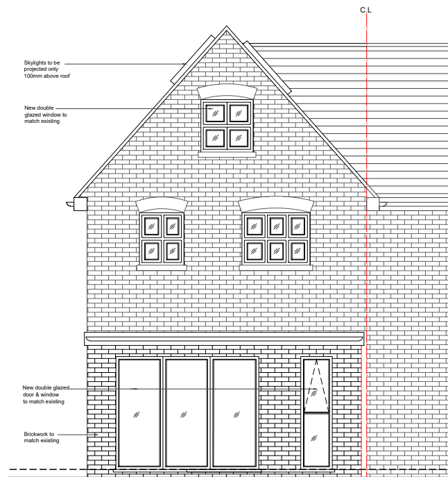
04 - REAR ELEVATION
