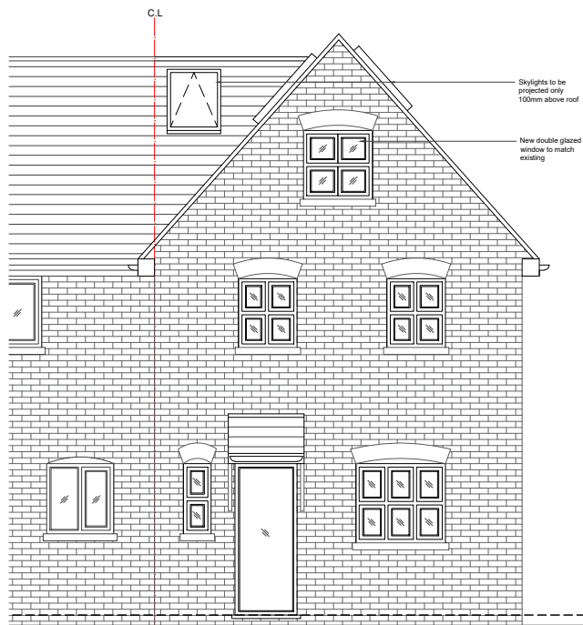
03 - FRONT ELEVATION
