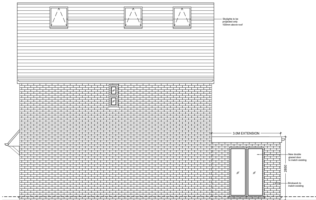
05 - SIDE ELEVATION
