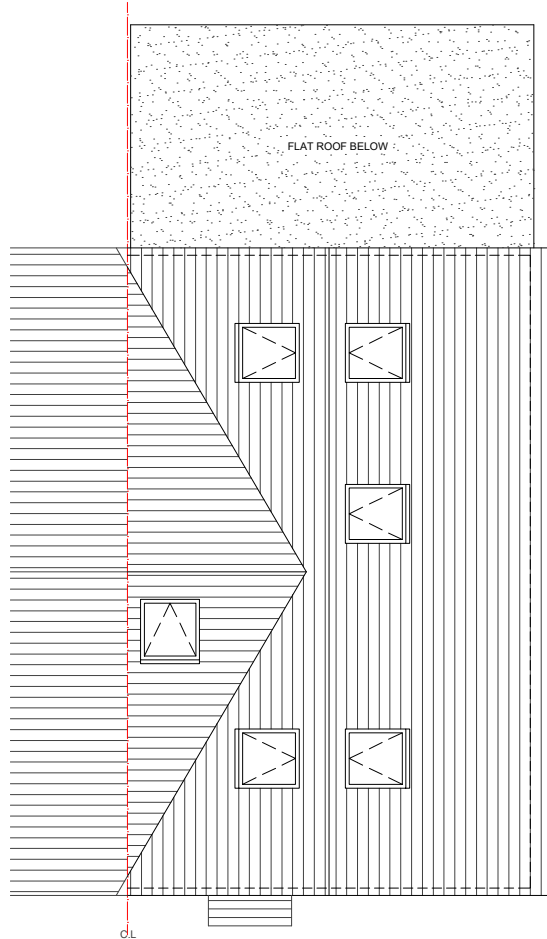
02 - ROOF PLAN
