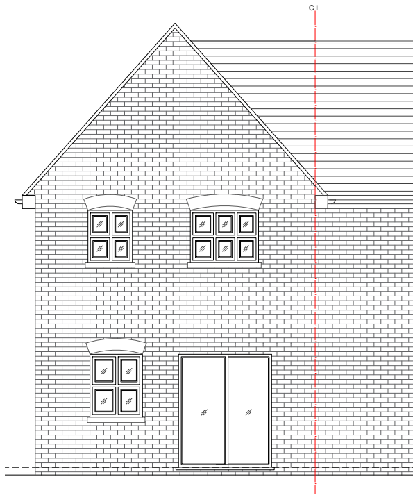
04 - REAR ELEVATION
