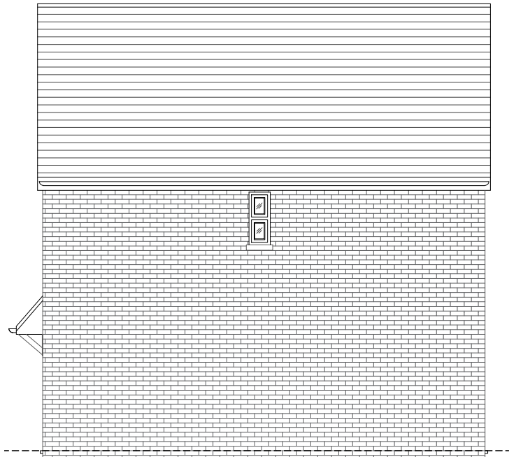
05 - SIDE ELEVATION
