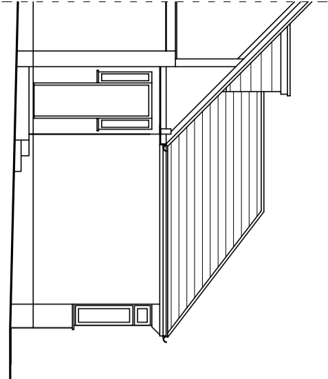
SECTION A-A SIDE ELEVATION PROPOSED
