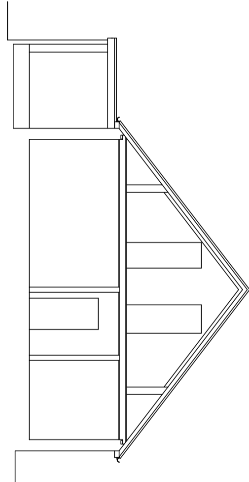
SECTION C-C PROPOSED
