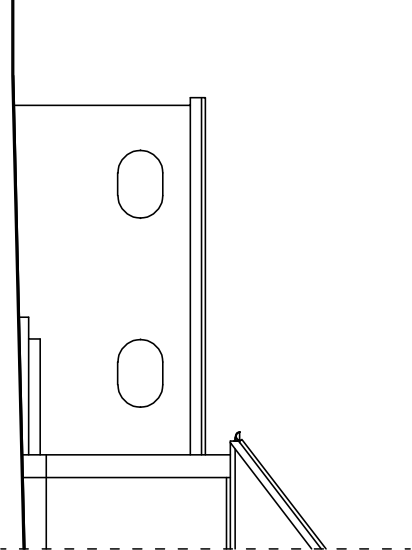
SECTION B-B SIDE ELEVATION EXISTING
