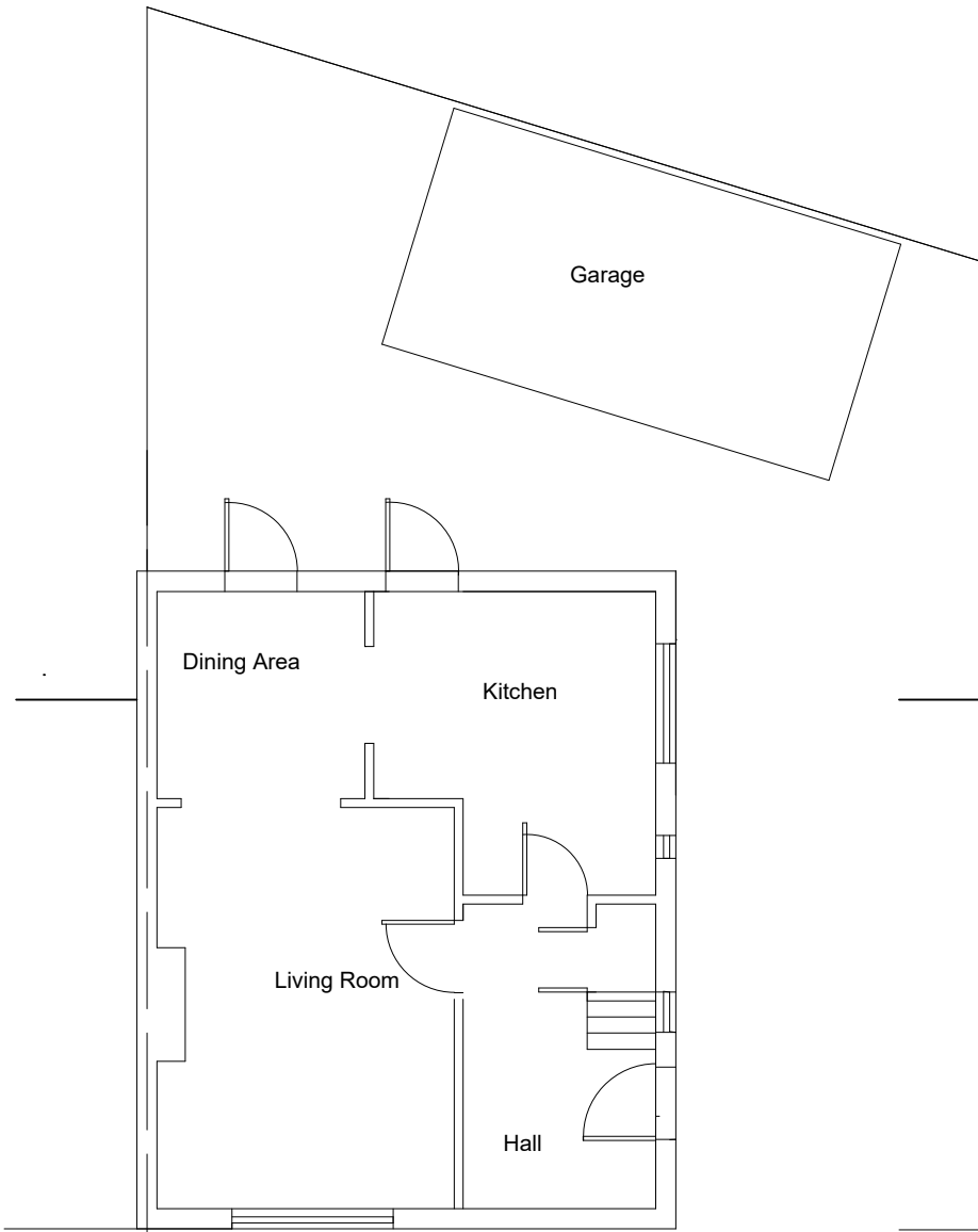
Ground Floor Plan as Existing
