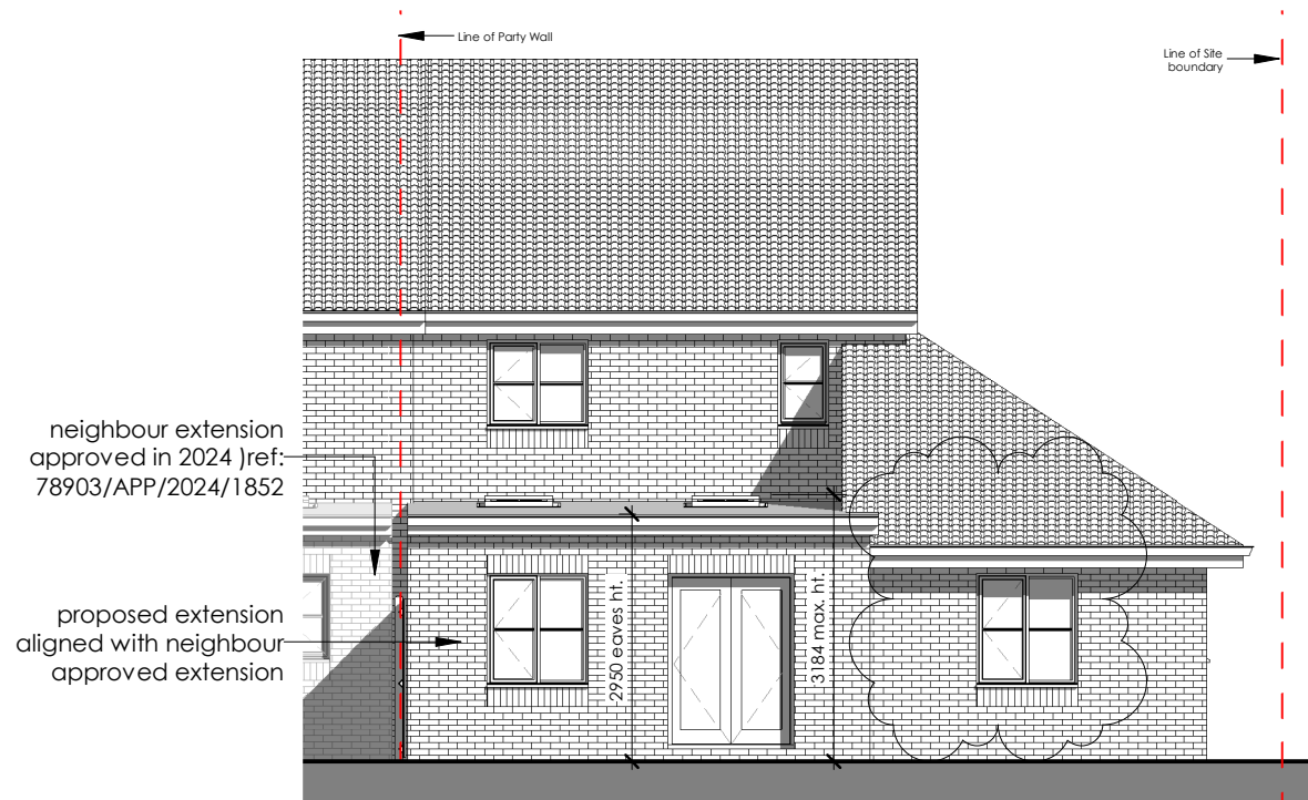
3 Proposed Rear Elevation 2508-A-201 1 : 100
