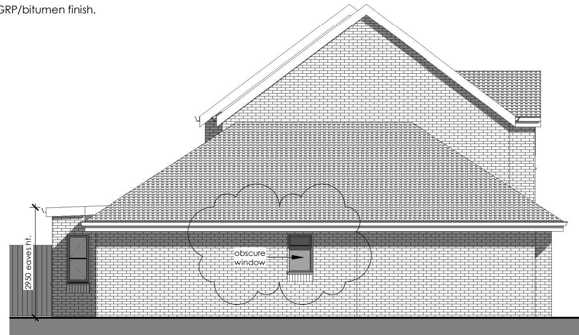
4 Proposed Side Elevation 2 2508-A-201 1 : 100
