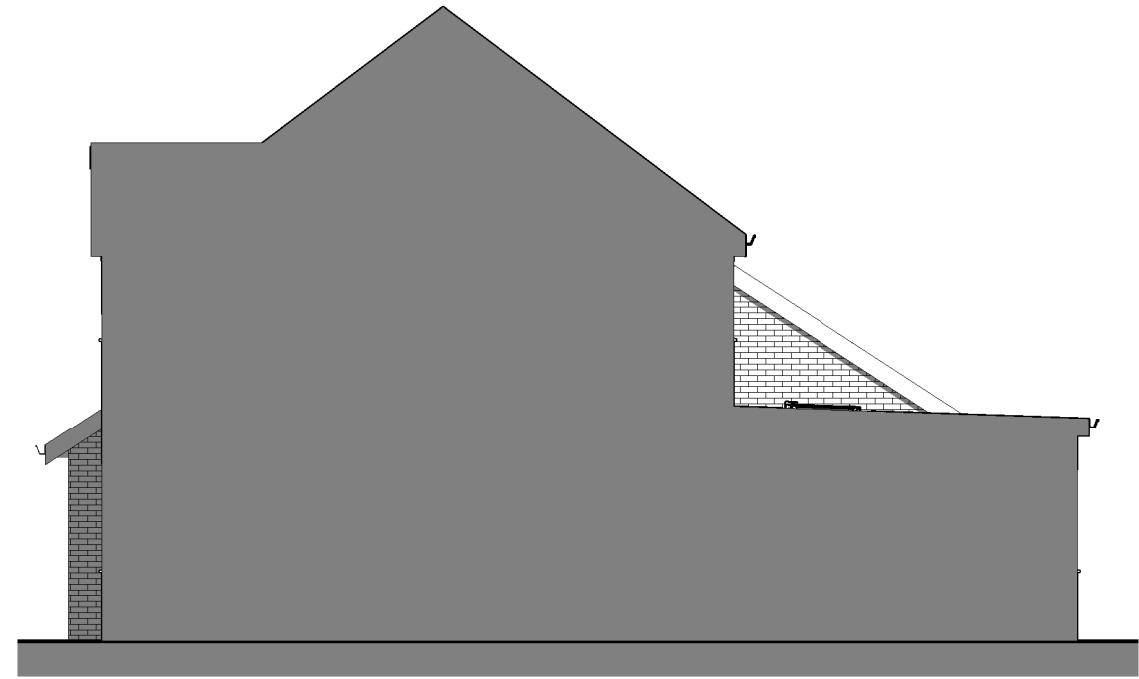
2 Proposed Side Elevation 2508-A-201 1 : 100
