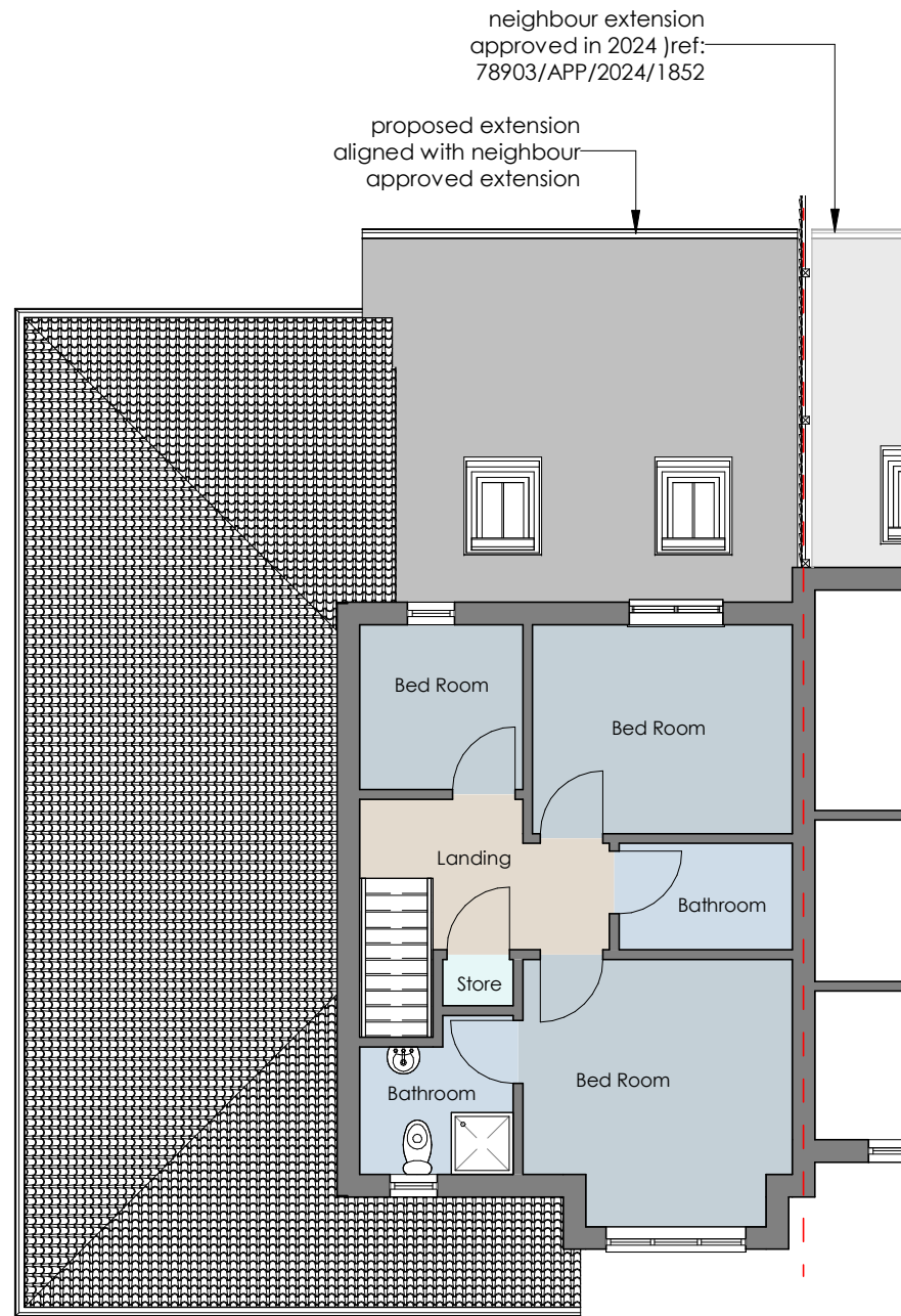
5 Proposed First Floor 2508-A-200 1 : 100
