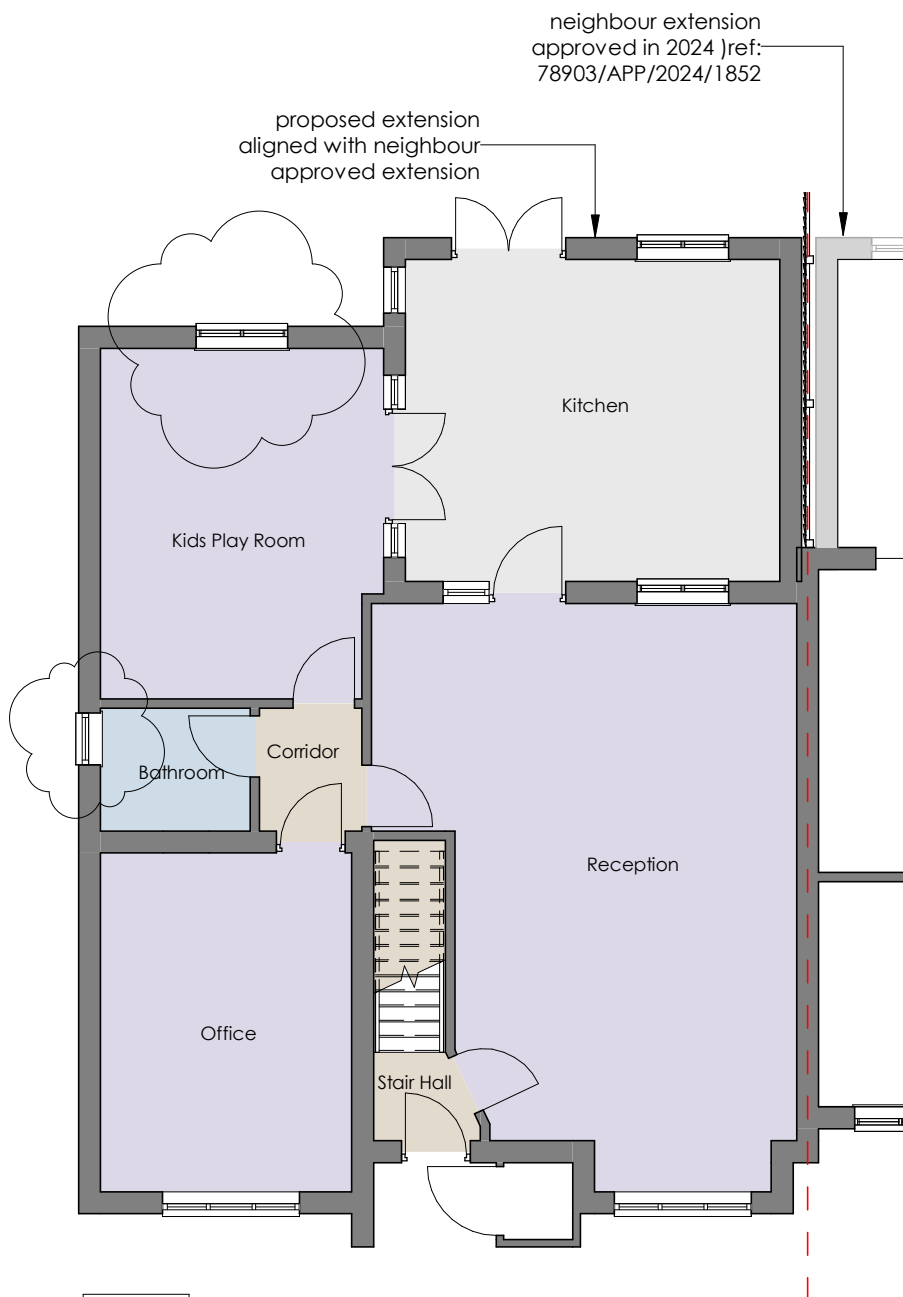
4 Proposed Ground Floor 2508-A-200 1 : 100
