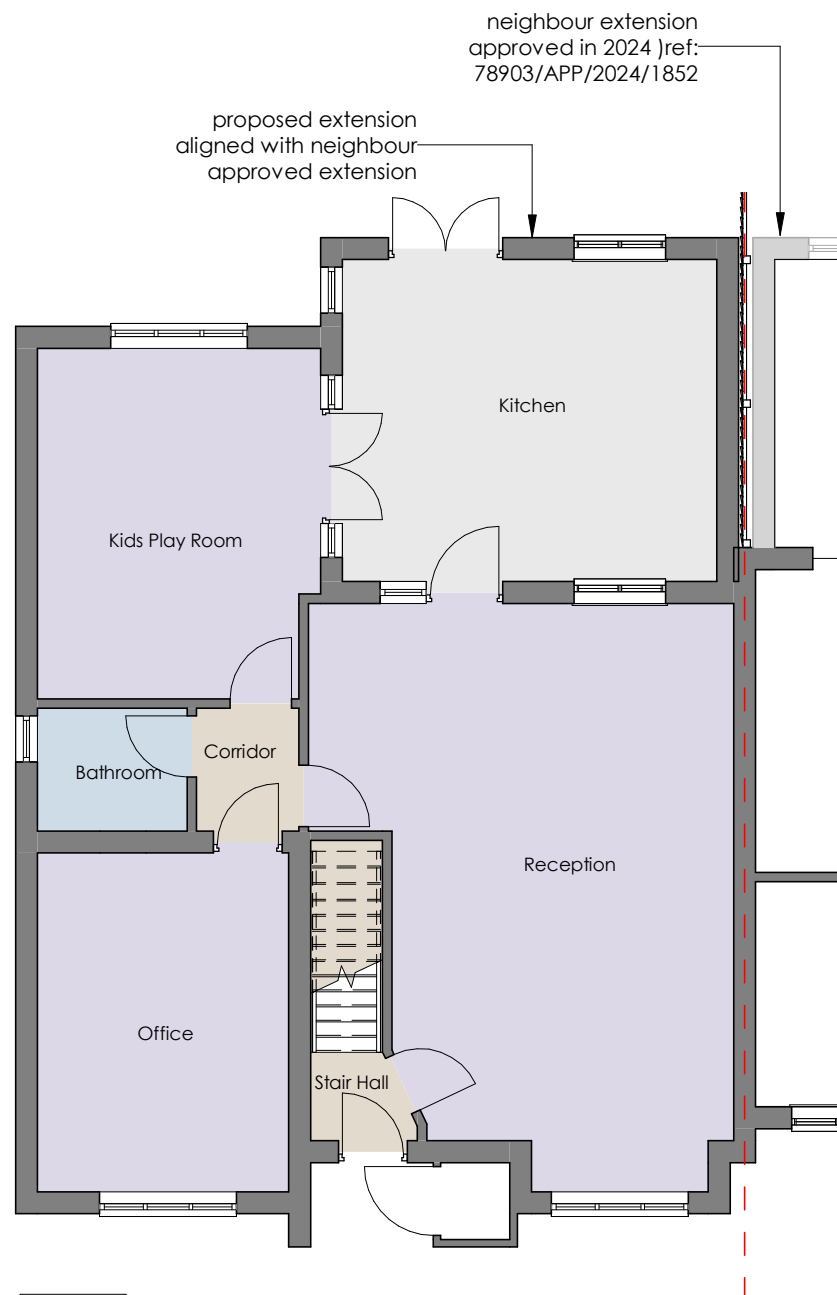
4 Proposed Ground Floor 2508-A-200 1 : 100
