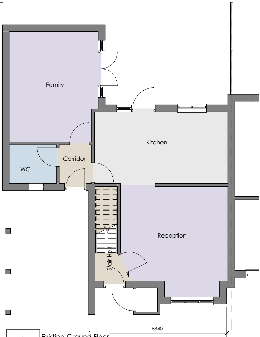
1 Existing Ground Floor 2508-A-100 1 : 100
