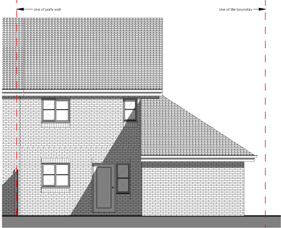
6 Existing Rear Elevation 2508-A-100 1 : 100
