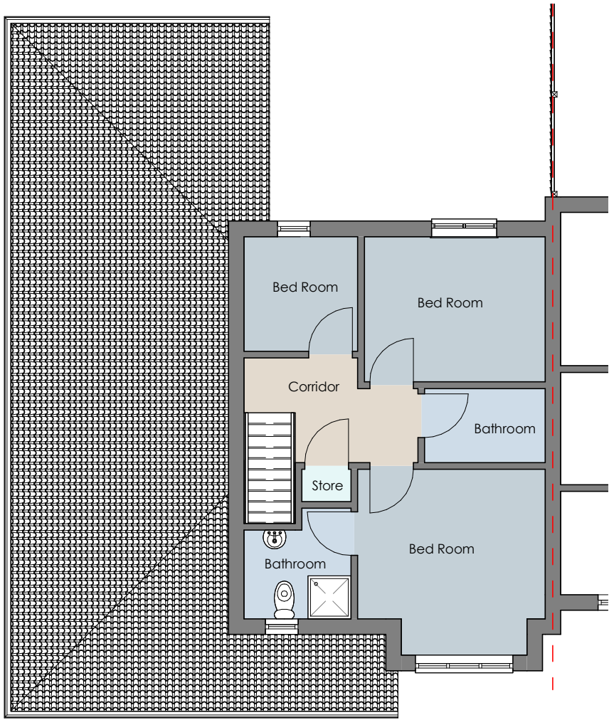
2 Existing First Floor 2508-A-100 1 : 100
