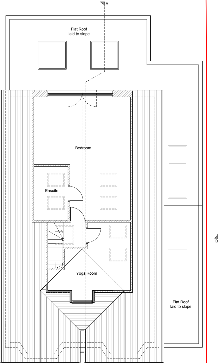
PROPOSED FIRST FLOOR PLAN SCALE (m)
