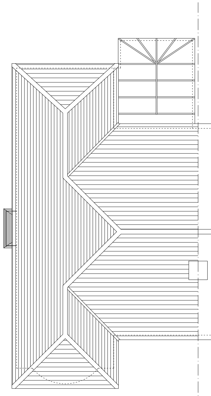
ROOF PLAN
