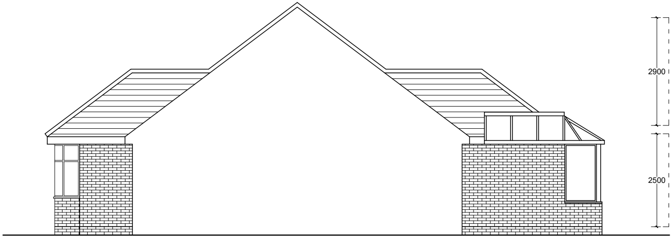
SIDE ELEVATION
