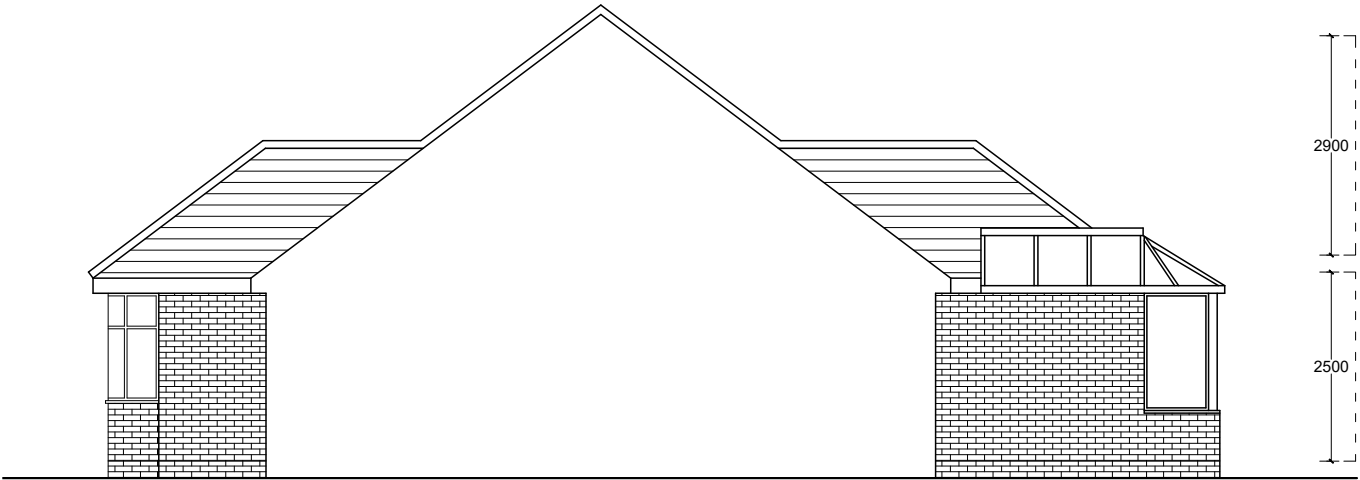
SIDE ELEVATION
