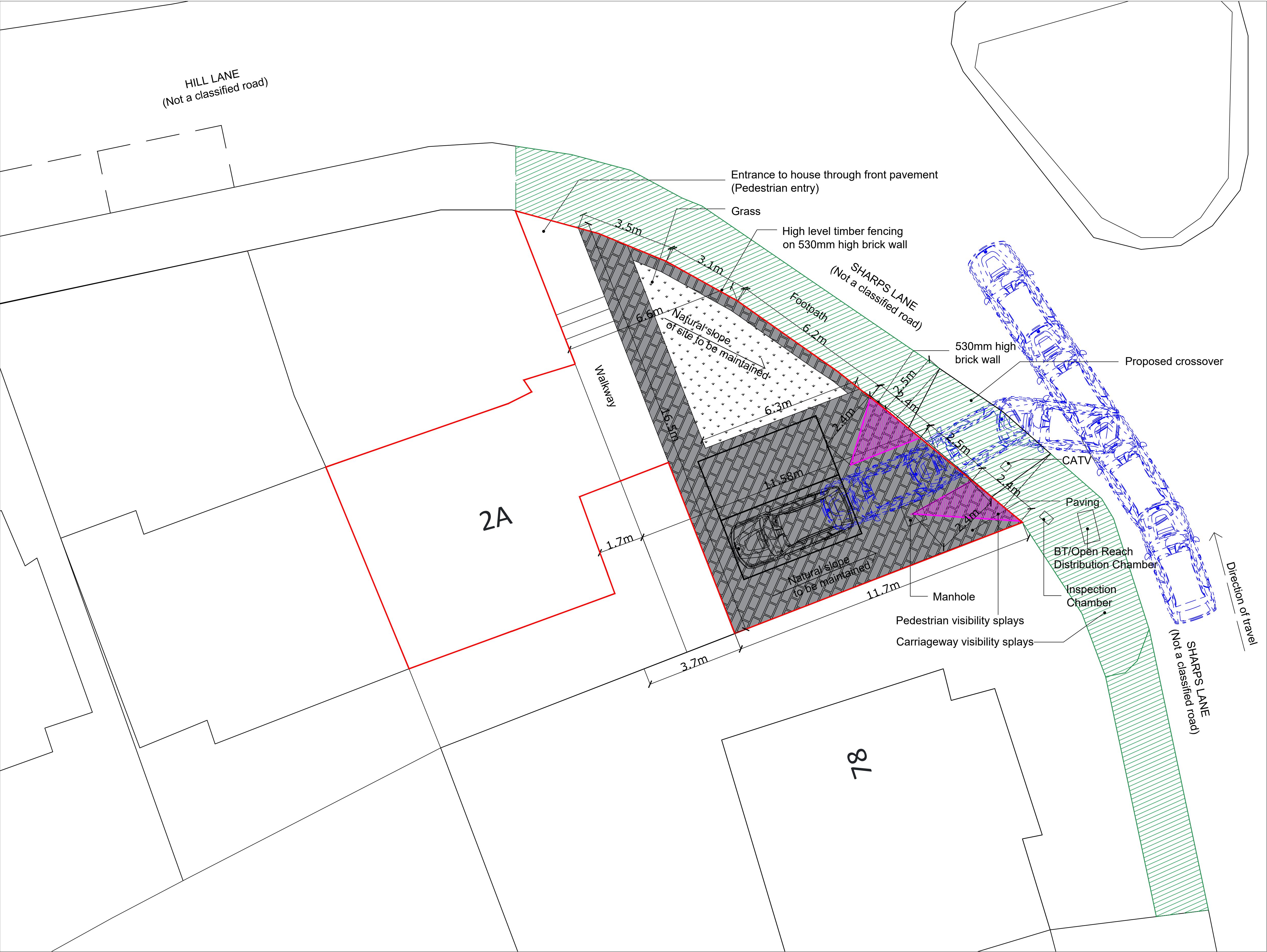
PROPOSED SITE EXIT PLAN
