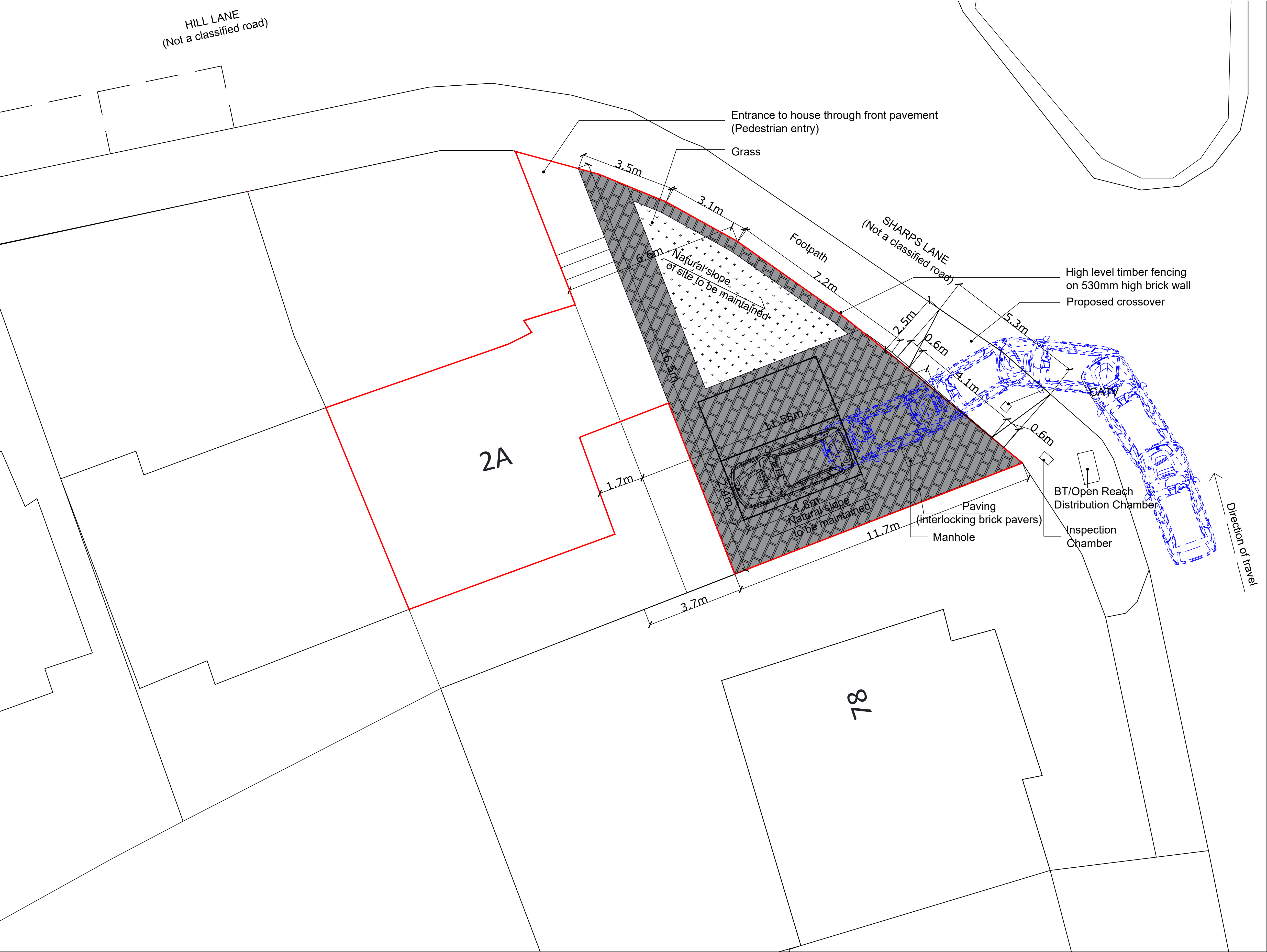
PROPOSED SITE ENTRY PLAN
