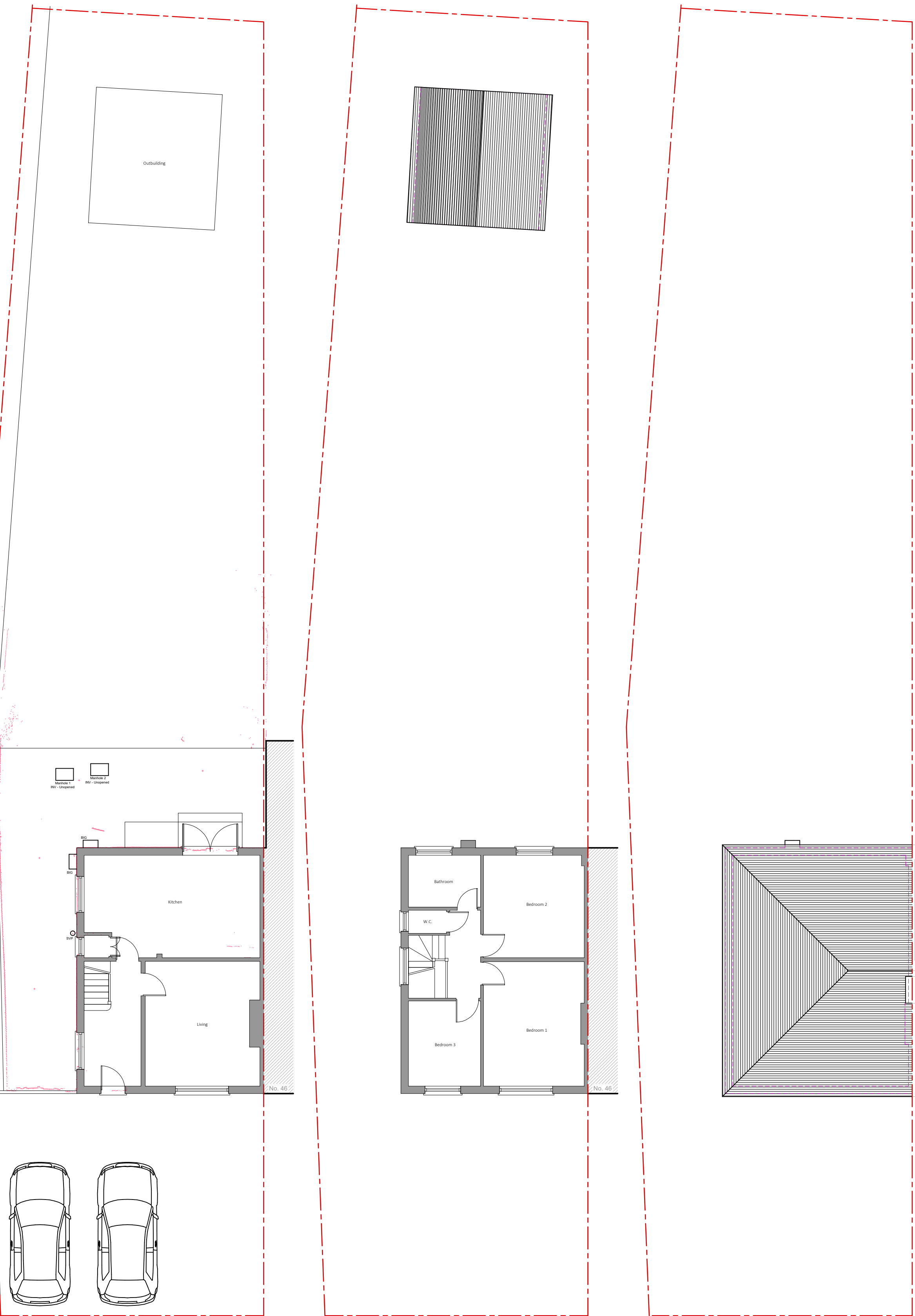
1 Existing Ground Floor Plan
