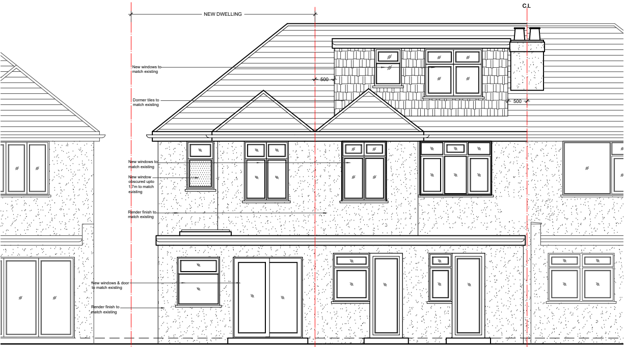
03 - REAR ELEVATION
