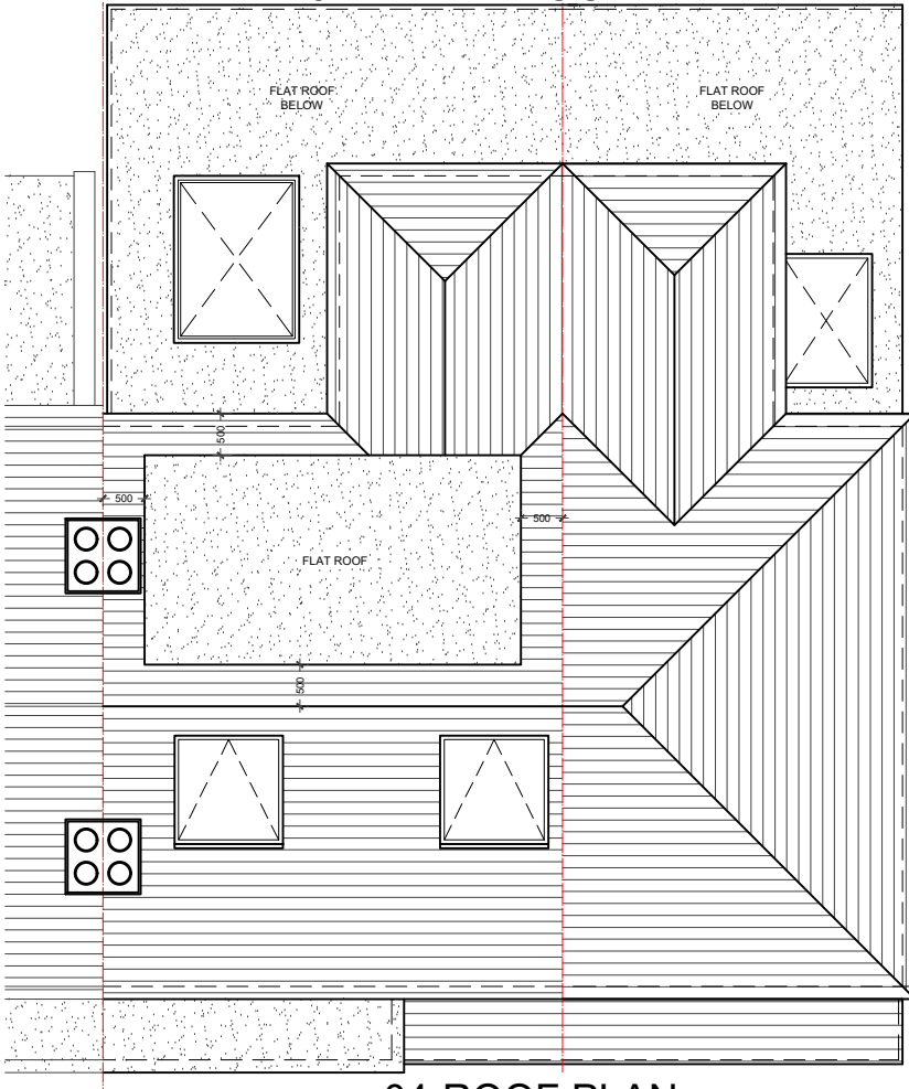
04-ROOF PLAN
