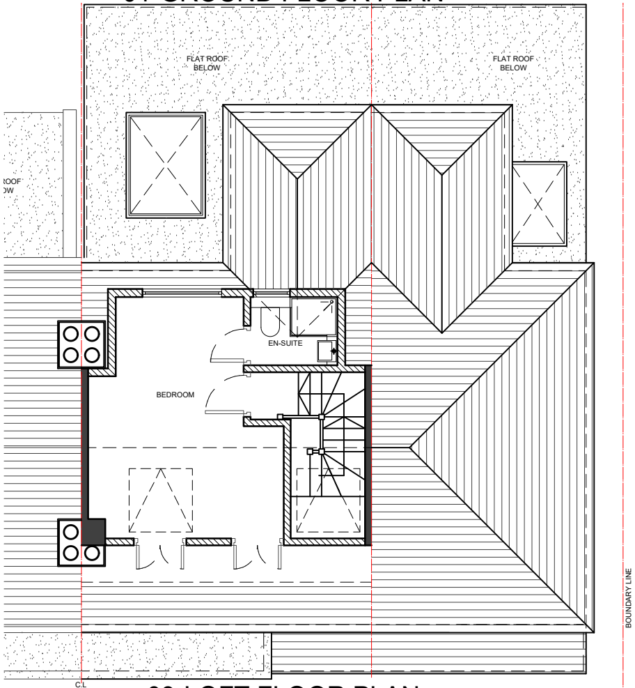
03-LOFT FLOOR PLAN
