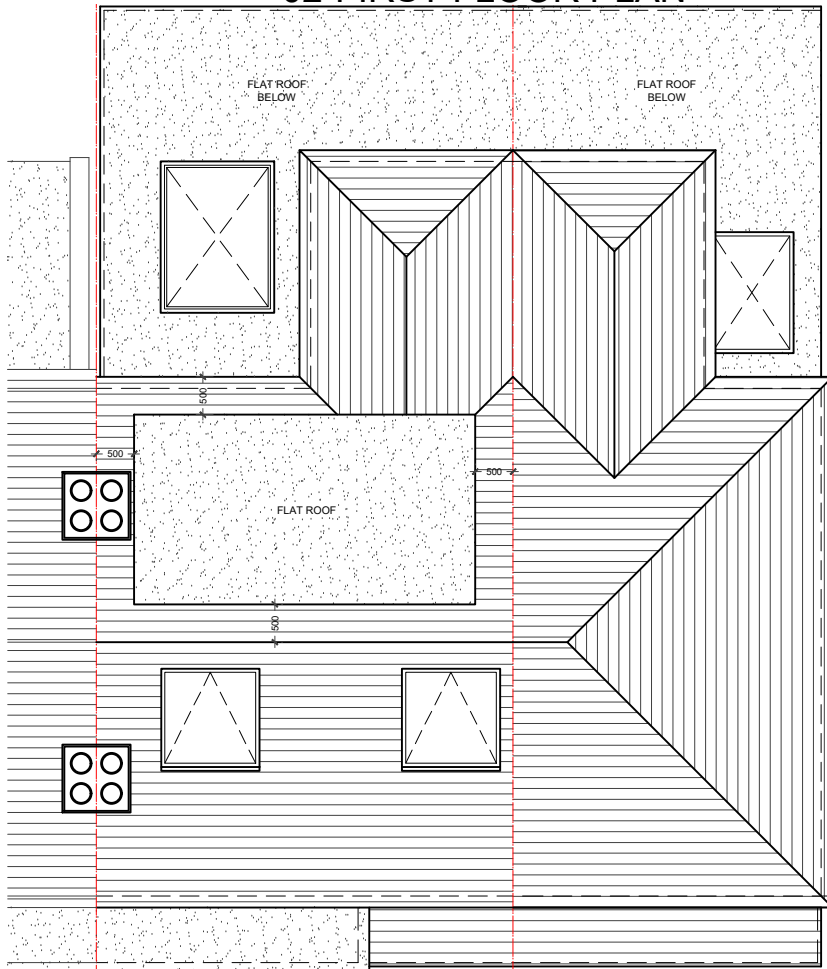
04-ROOF PLAN
