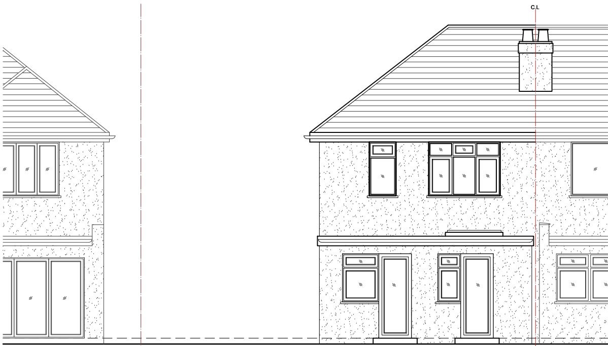
03 - REAR ELEVATION
