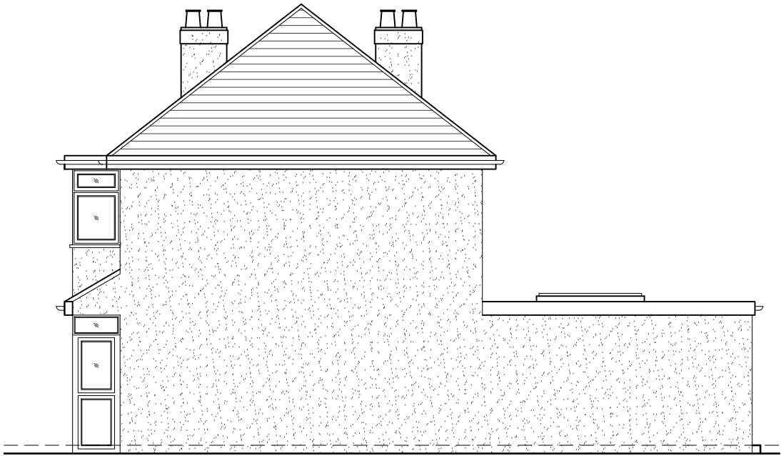
02 - SIDE ELEVATION
