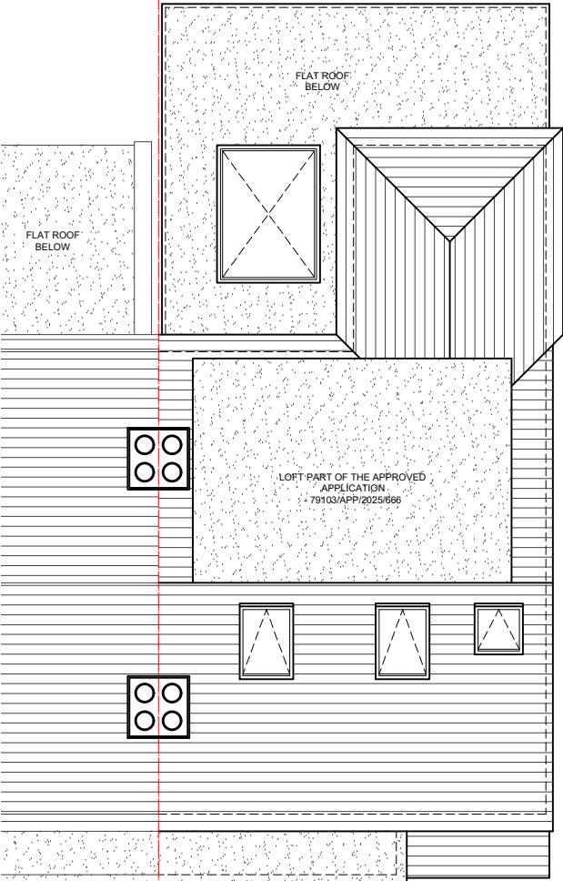
04 - ROOF PLAN
