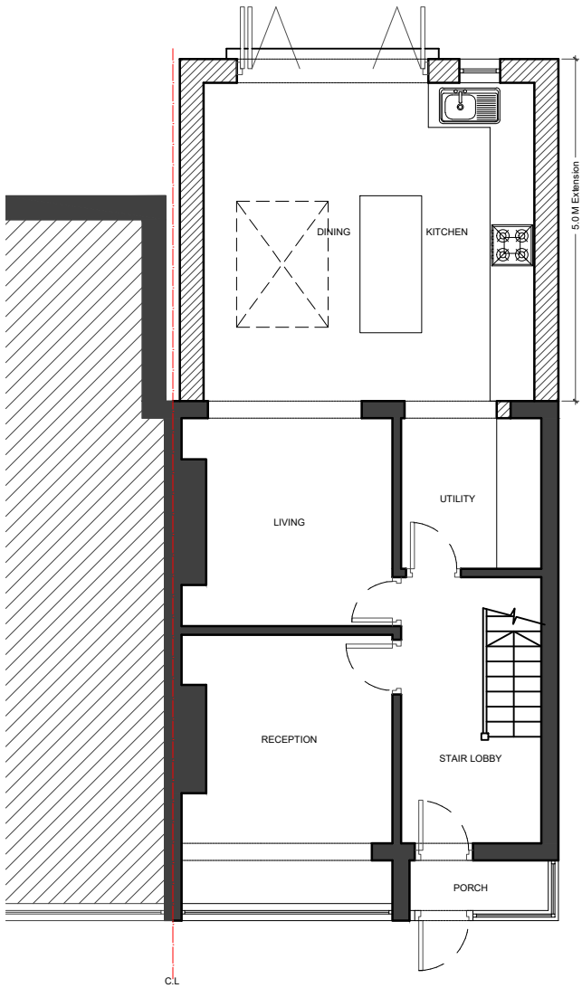
01 - GROUND FLOOR PLAN
