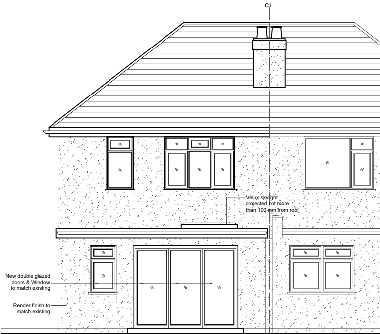
04 - REAR ELEVATION
