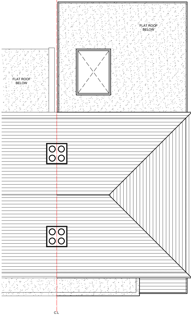
02 - ROOF PLAN
