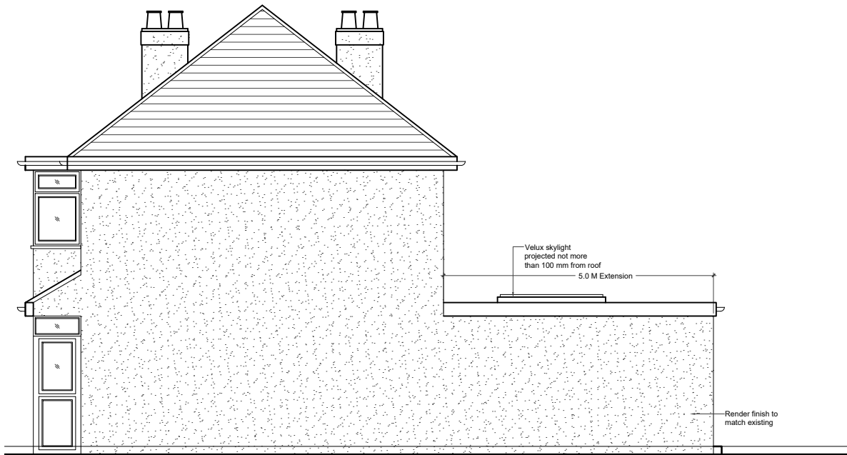
03 - SIDE ELEVATION
