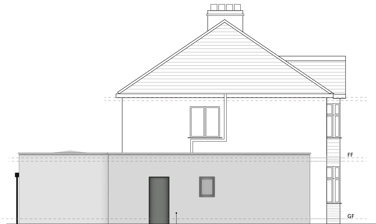
1 SOUTH WEST - FRONT
