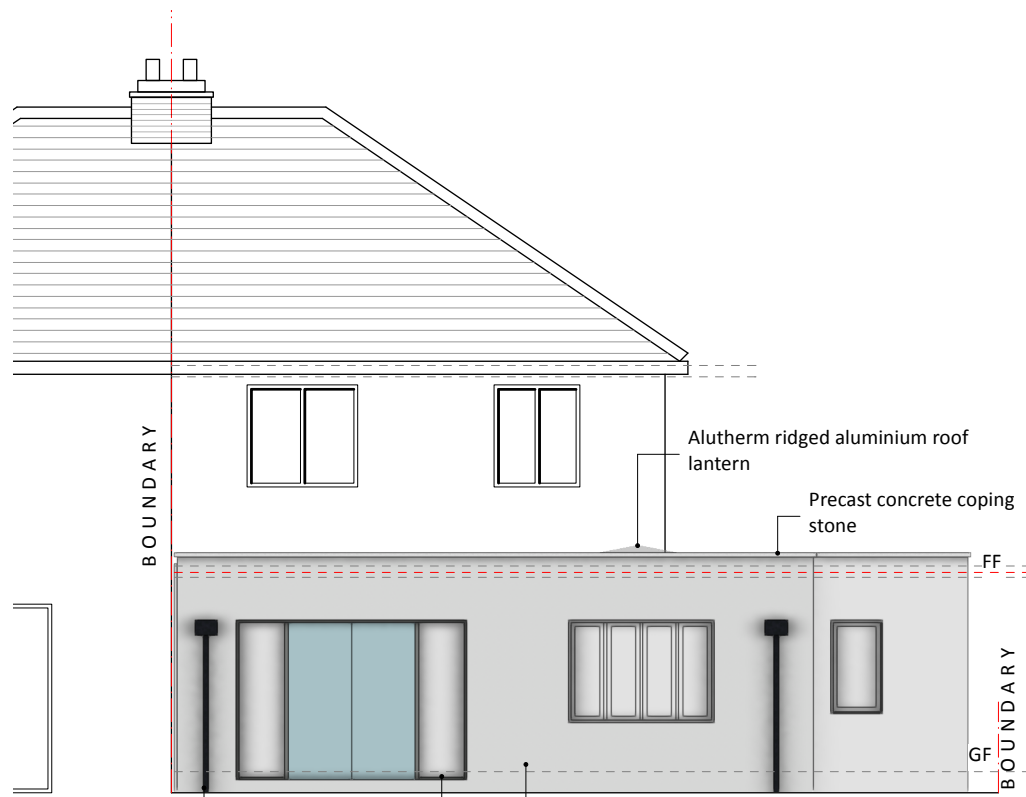
2 SOUTH EAST - SIDE
