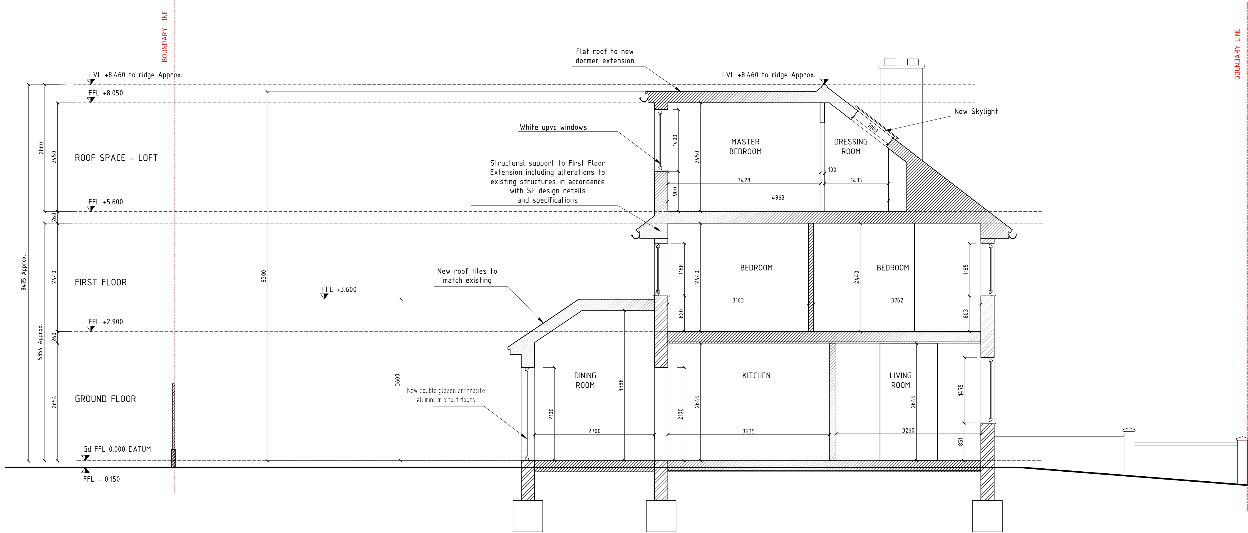
PROPOSED SECTION A - A (SCALE 1:50@A1)
