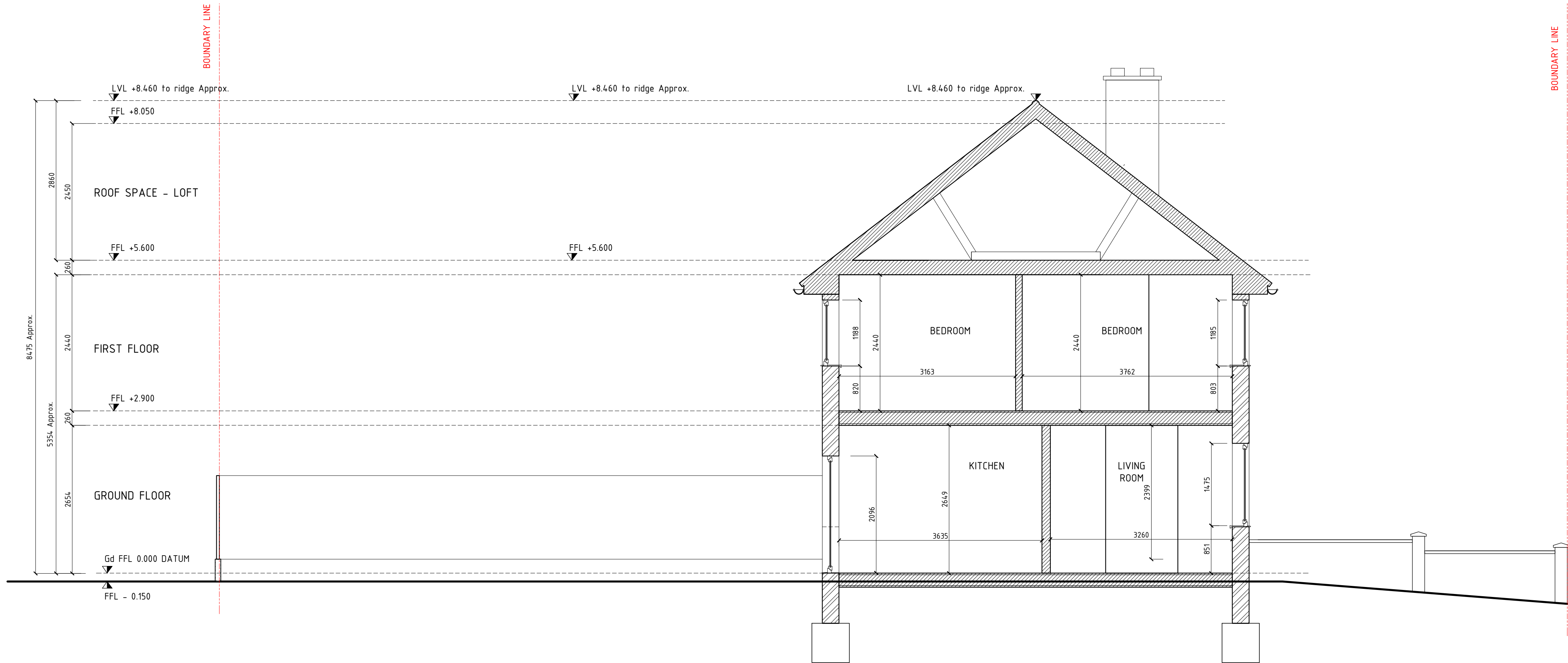
EXISTING SECTION A - A (SCALE 1:50@A1)
