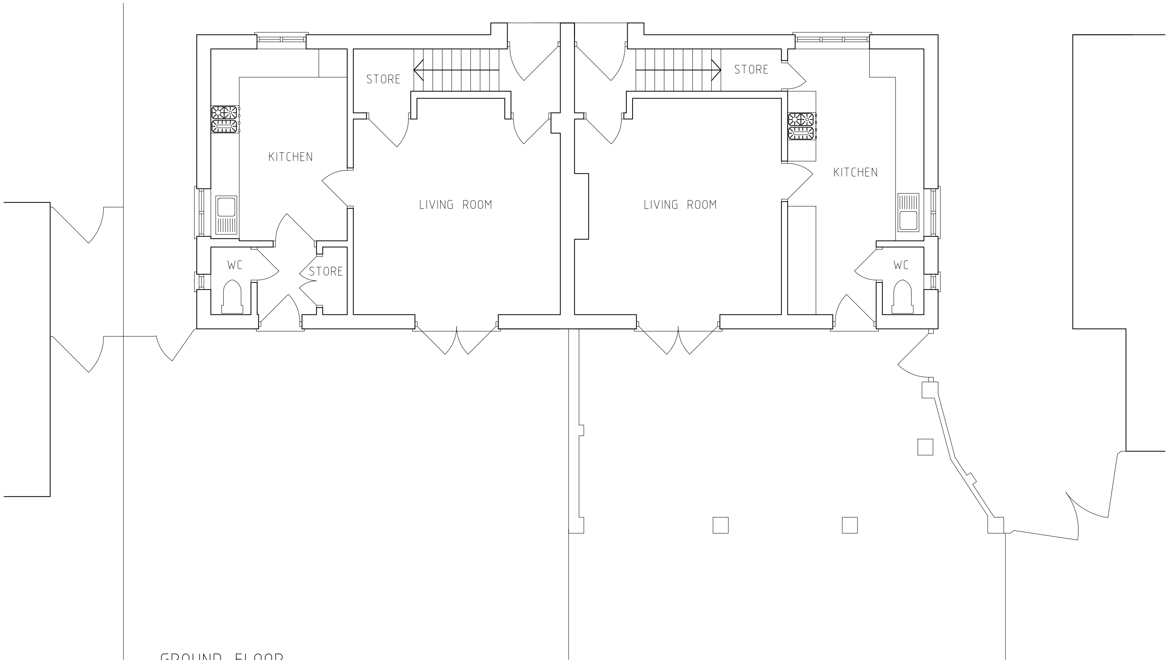
GROUND FLOOR
