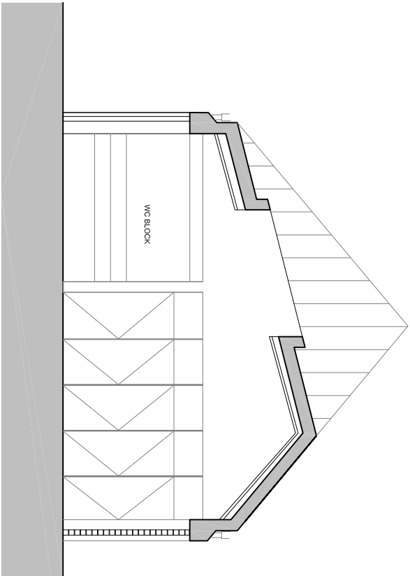
BB Short Section - Through WC Block
