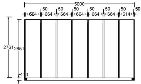
Existing and Proposed Floor/Elevation Plans
