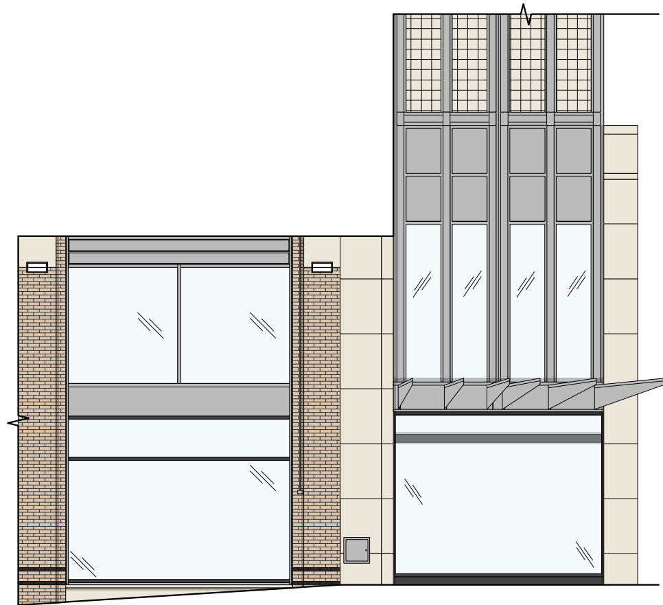
EXISTING ELEVATIONS
