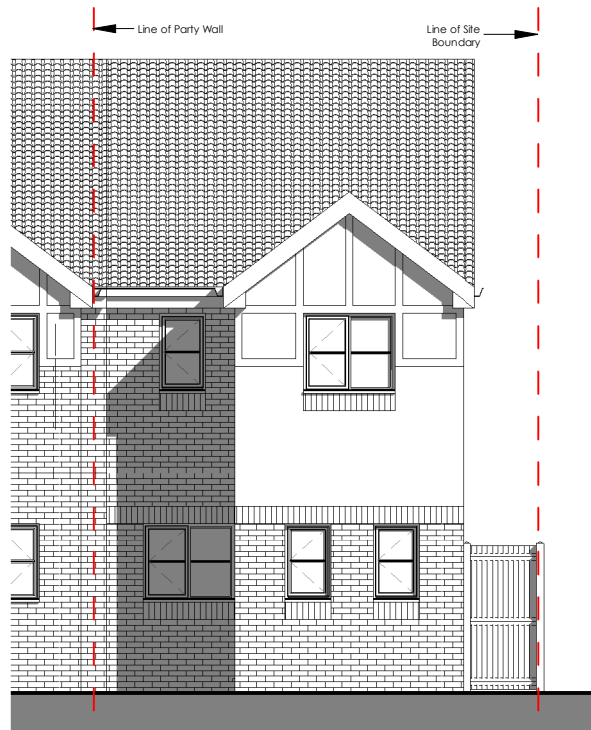
1 Proposed Front Elevation 2422-A-250 1 : 100
