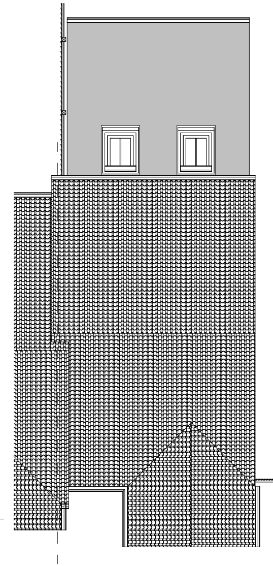
3 Proposed Rear Elevation 2422-A-250 1 : 100
