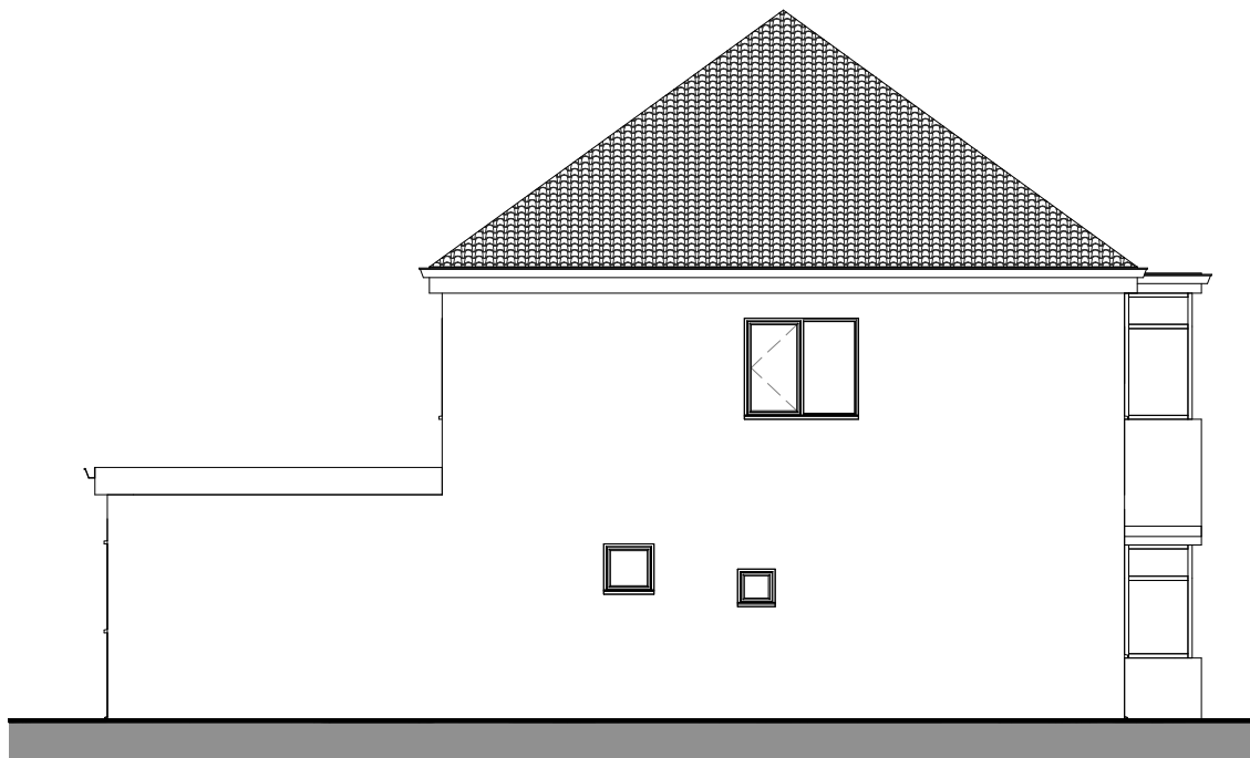
5 Existing Side Elevation 2424-A-101 1 : 100
