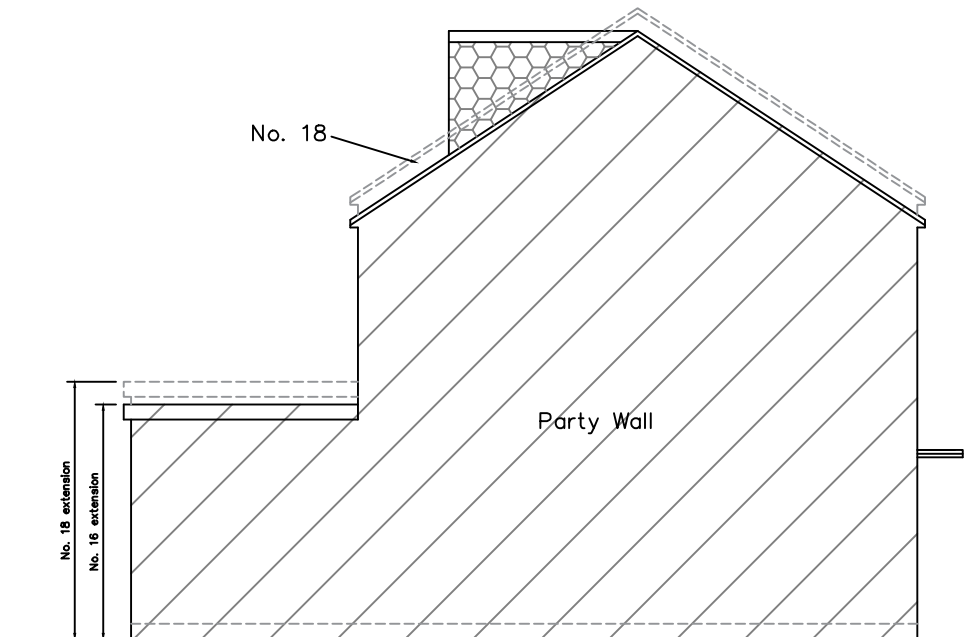
Proposed Side Elevation View D
