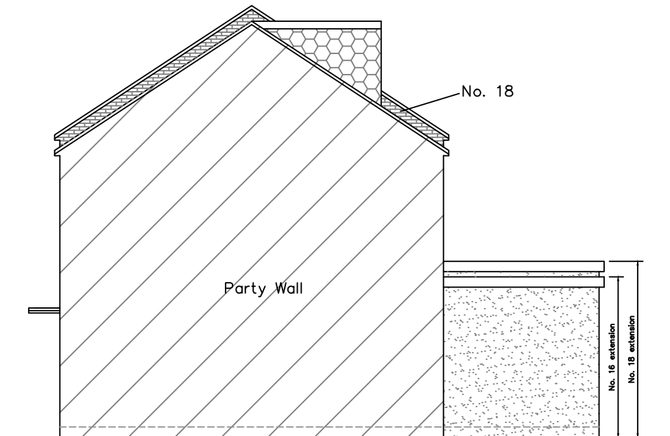
Proposed Side Elevation View C
