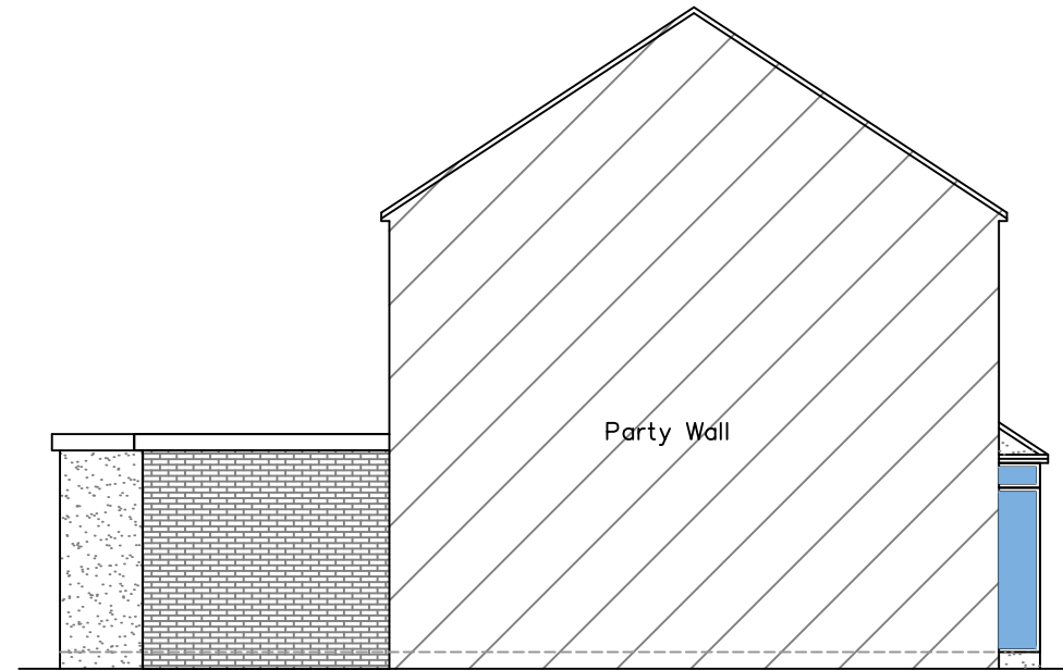
Proposed Side Elevation View B
