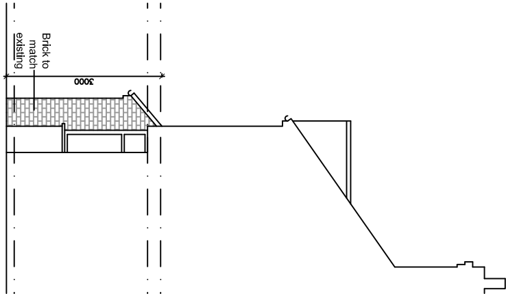
PROPOSED SECTIONAL SIDE ELEVATION
