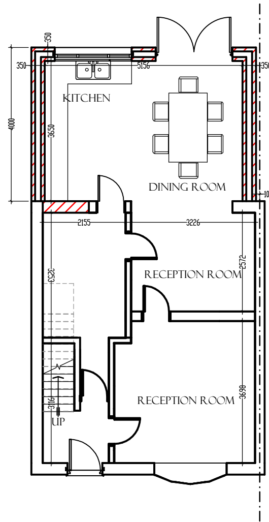
PROPOSED G.F PLAN
