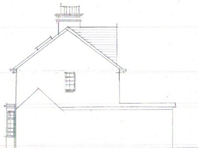
EAST ELEVATION
