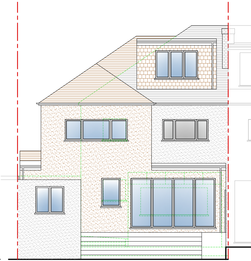
7 Proposed Rear Elevation
