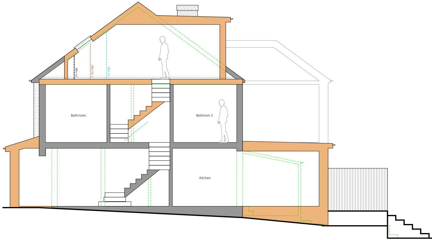
9 Proposed Side Section
