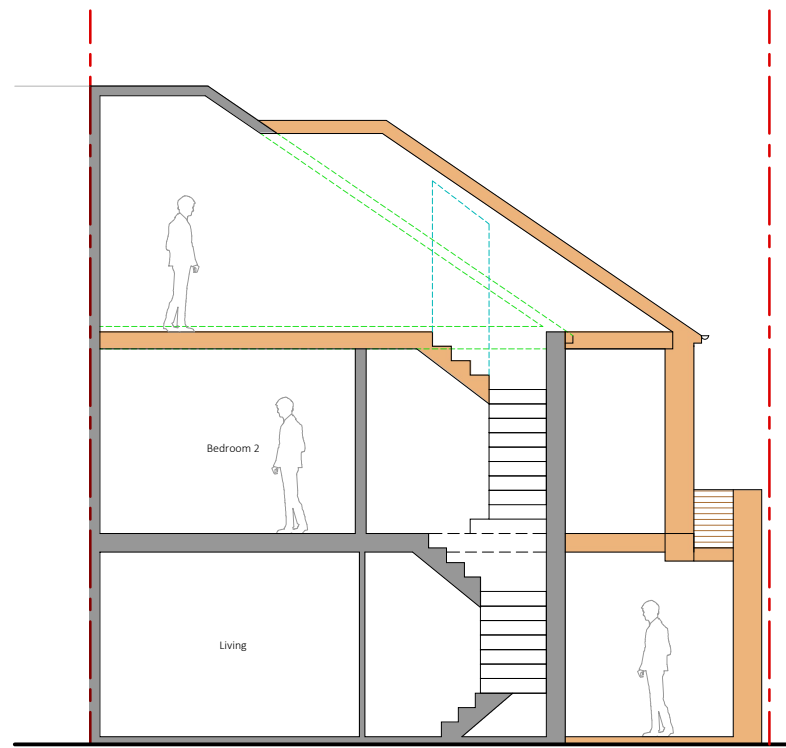
10 Proposed Front Section
