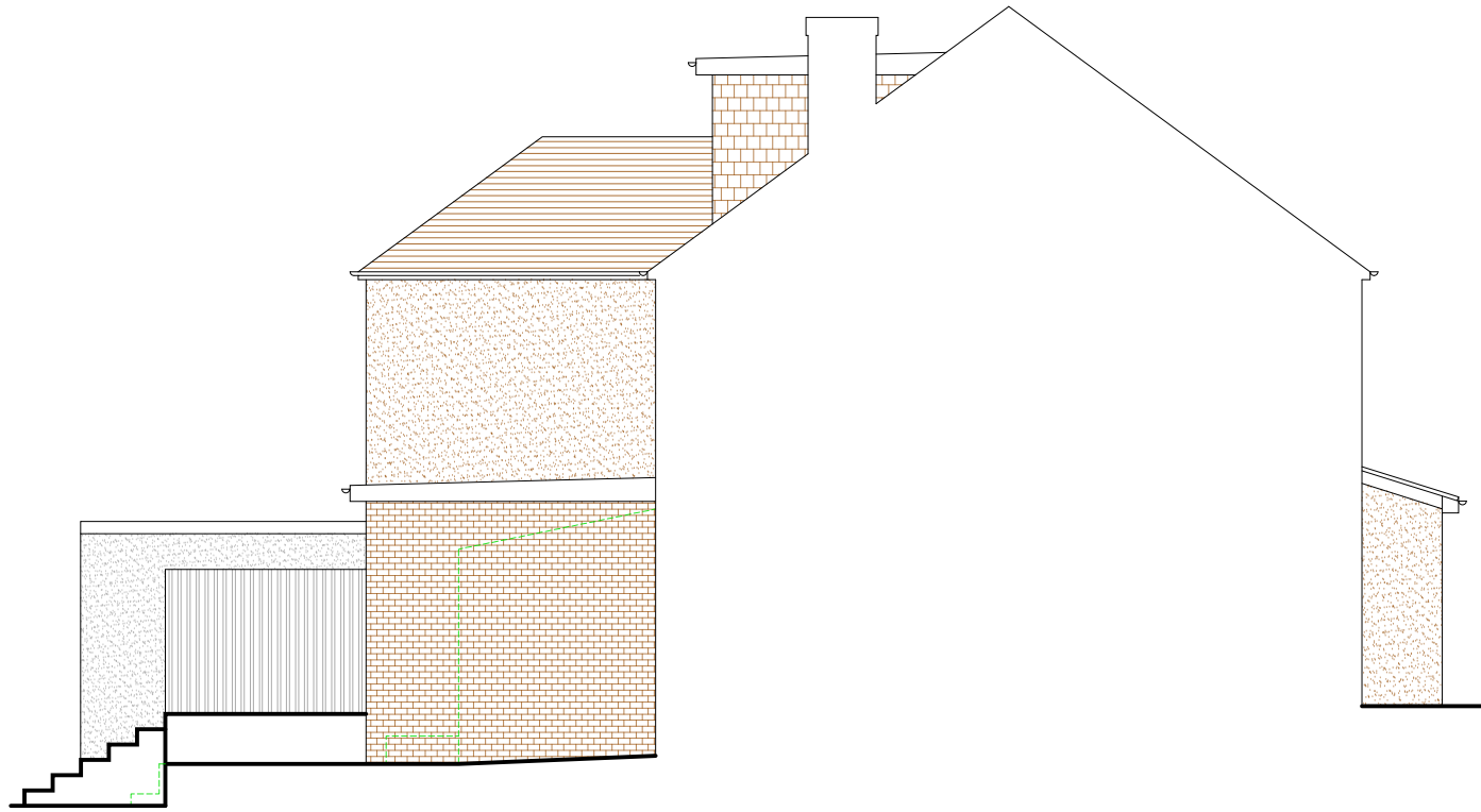
8 Proposed Side Elevation
