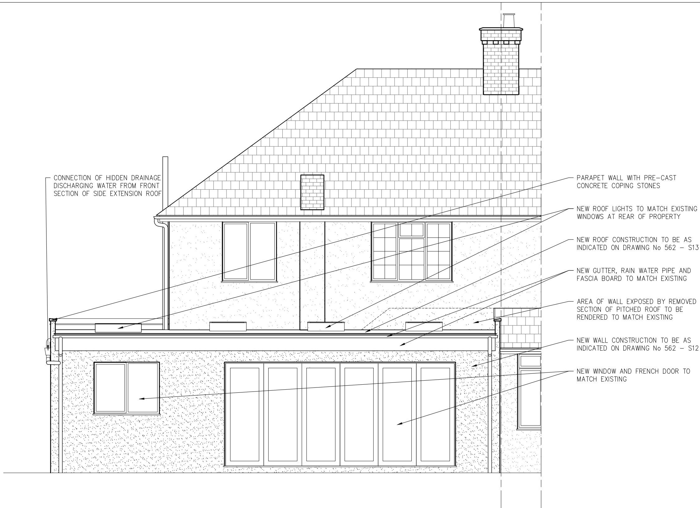
PROPOSED REAR ELEVATION SCALE 1:50
