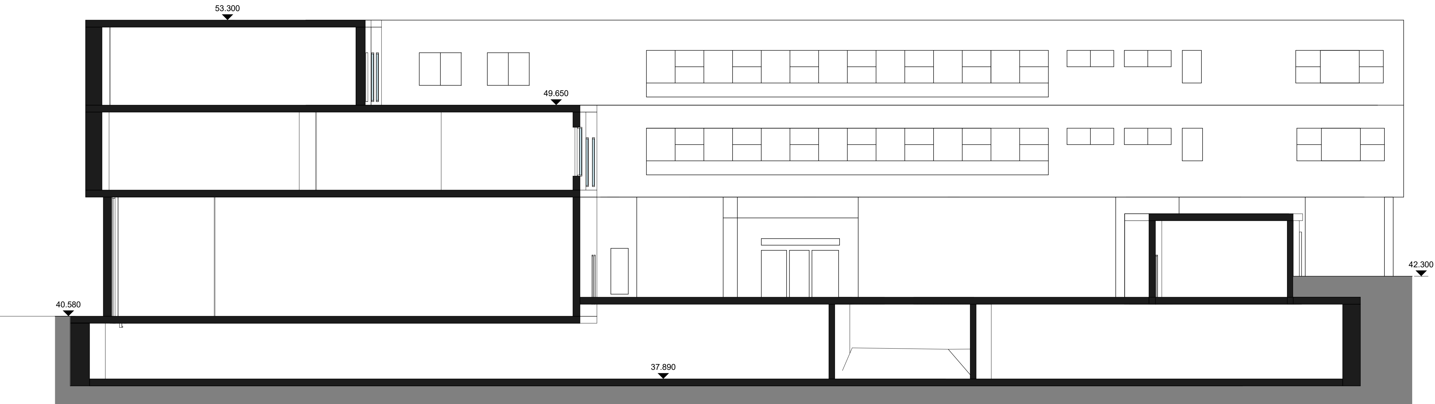
2 West Courtyard Elevation - Existing 1:100
