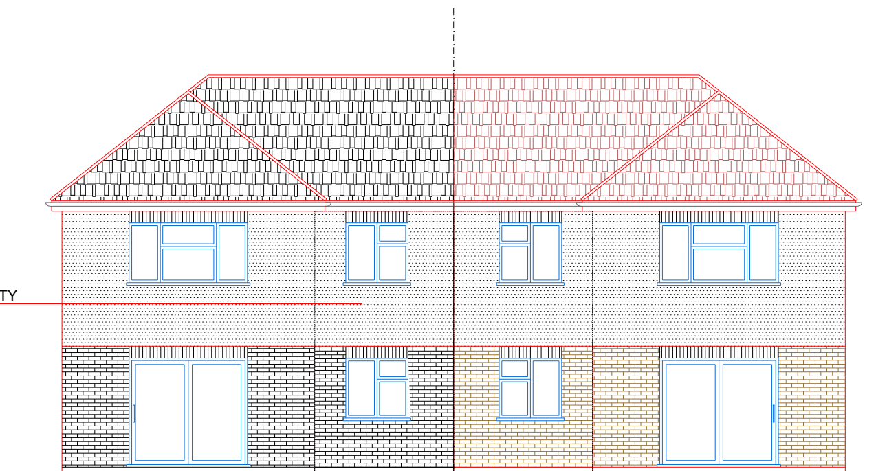
15 GREAT CENTRAL PROPOSED REAR ELEVATION
