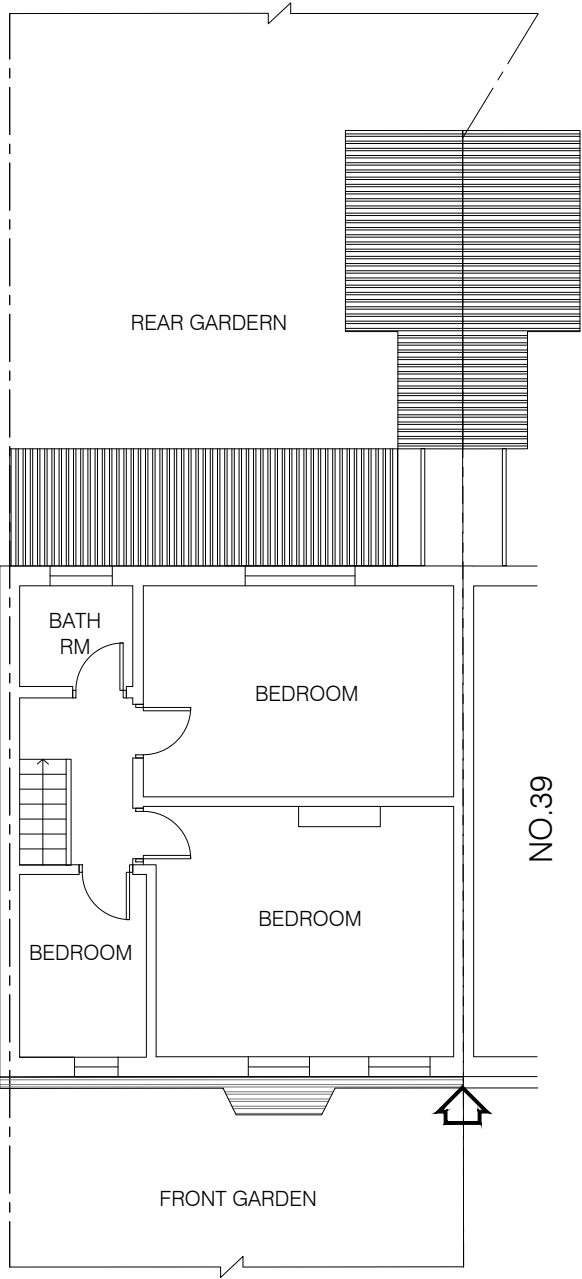
FF PLAN
