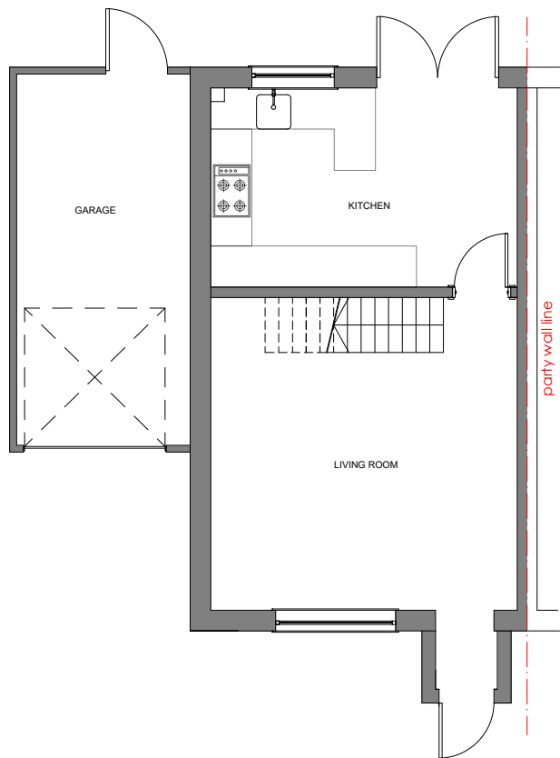
GROUND FLOOR PLAN - EXISTING
