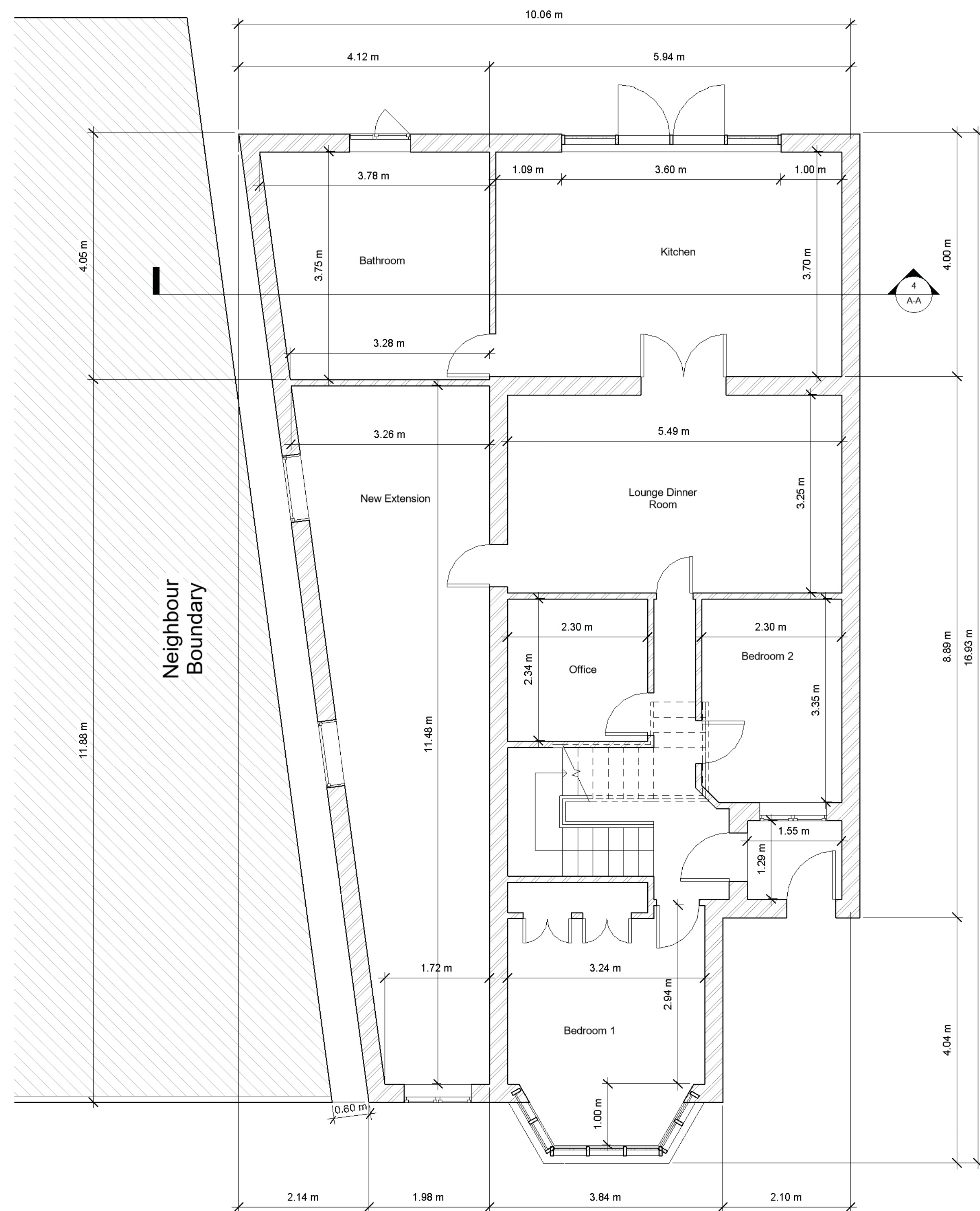
Ground Floor
