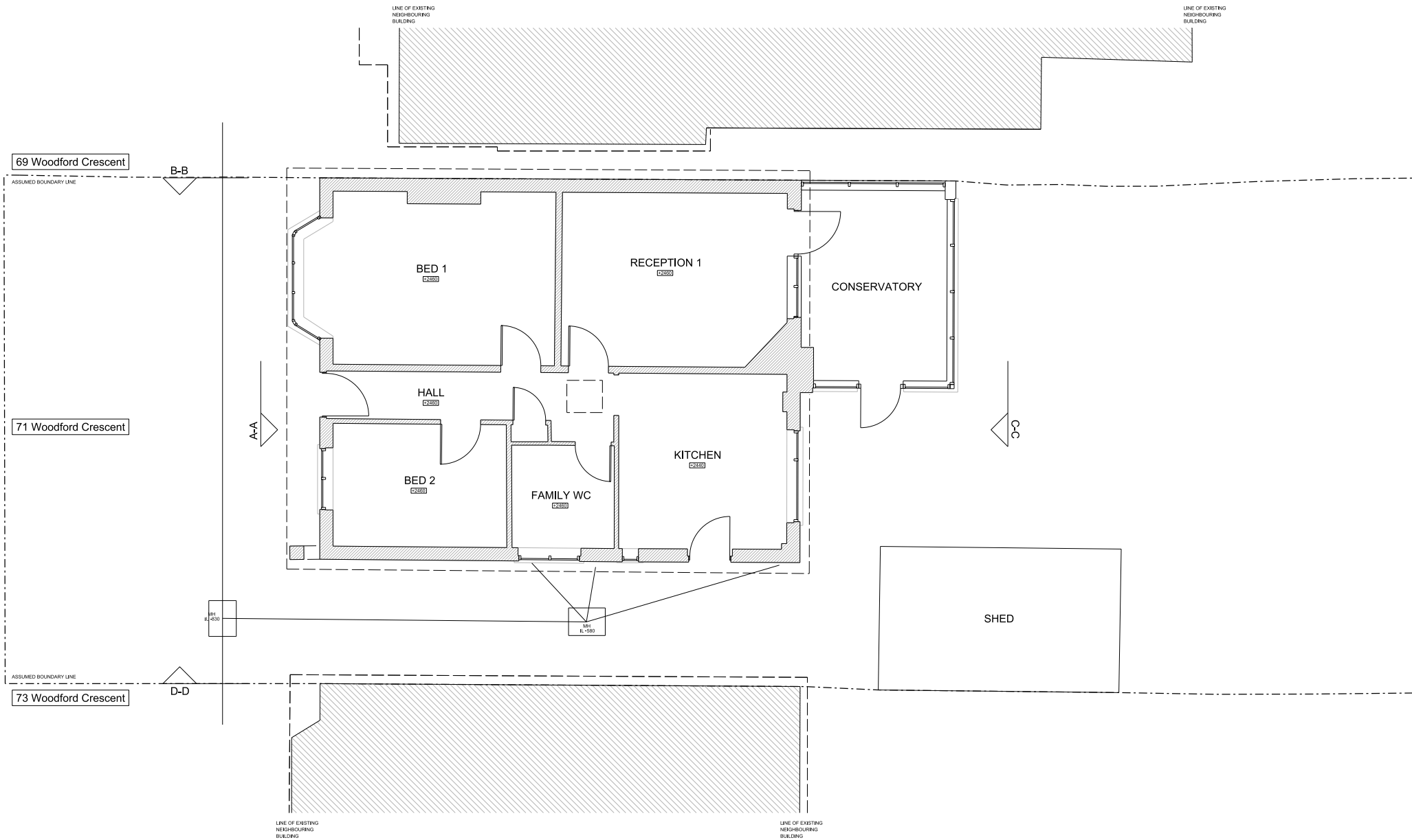
1. EXISTING GROUND FLOOR PLAN
