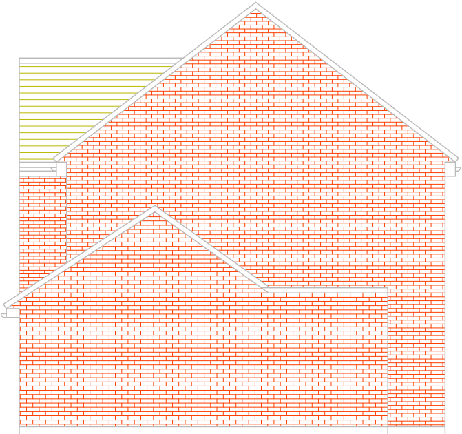
EXISTING SIDE ELEVATION-1
