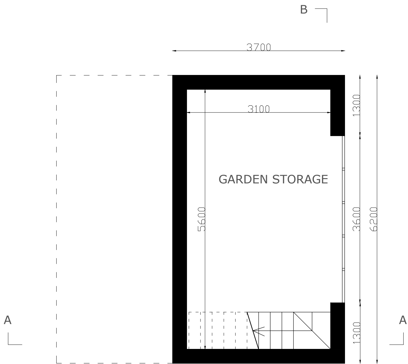
Storage/basement plan view
