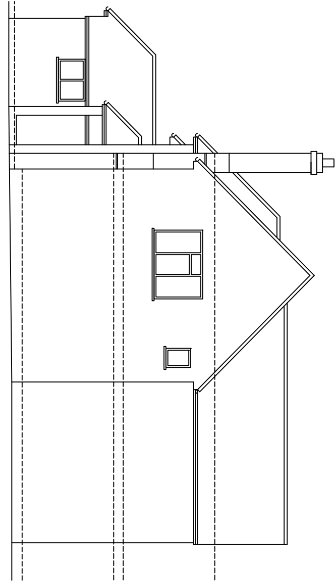
EXISTING SIDE ELEVATION 1
