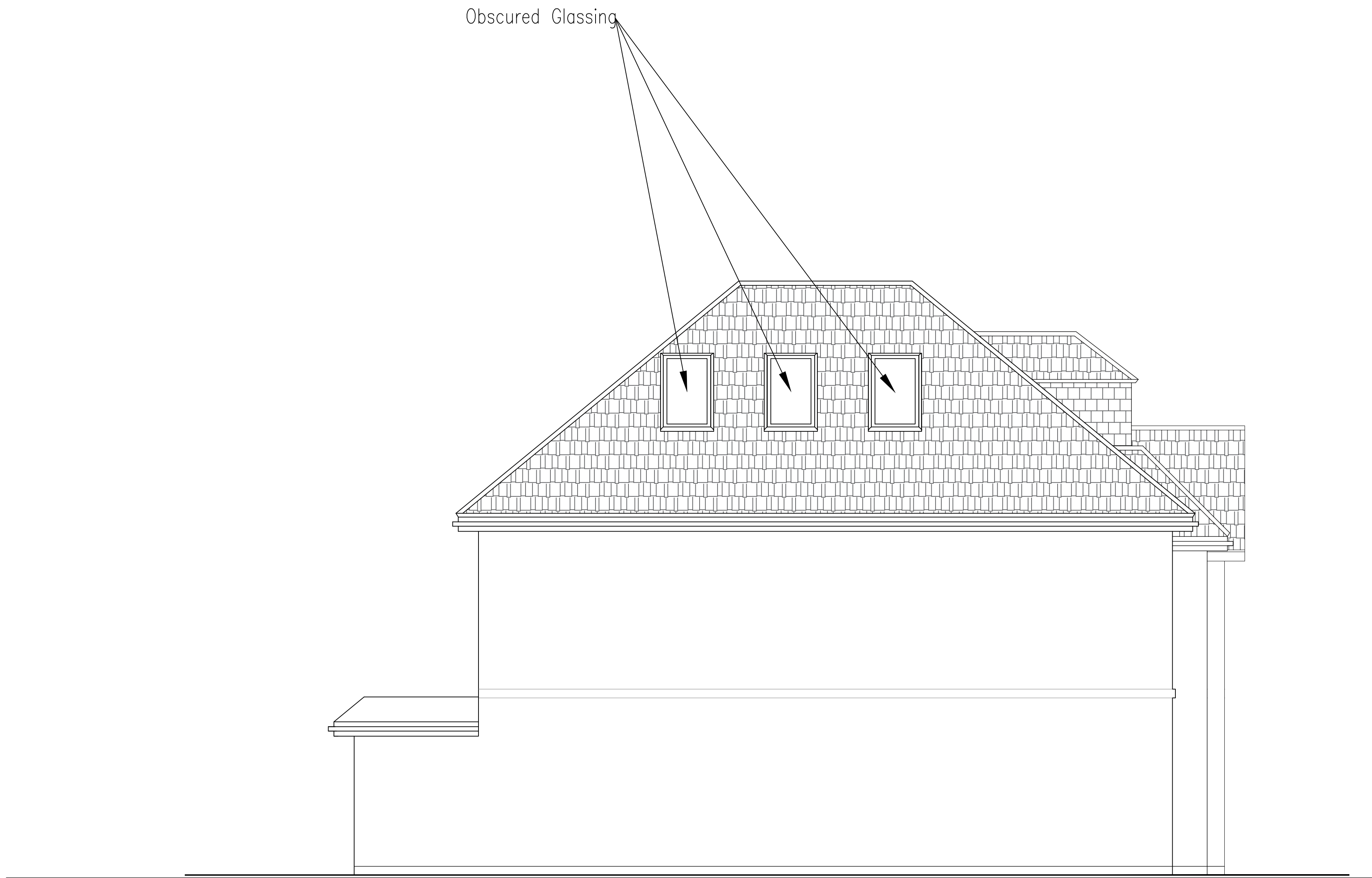
PROPOSED SIDE ELEVATION 1:50
